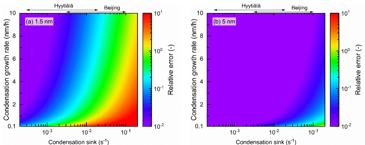
Figure A1 Error of the growth rate retrieved using the conventional appearance time method for (a) 1.5 nm and (b) 5 nm particles. The relative error is defined as (\text{GR}_{\text{conv}} - \text{GR}_{\text{cond}}) / \text{GR}_{\text{cond}} , where \text{GR}_{\text{conv}} is the growth rate retrieved by the conventional appearance time method and \text{GR}_{\text{cond}} is the condensation growth rate. Coagulation growth is neglected in this figure. The approximate range of condensation sink in Beijing (Wang et al., 2013) and Hyytiälä (Dal Maso et al., 2002) are marked with arrows, which indicate the typical condensation sink in polluted and clean environments, respectively.
