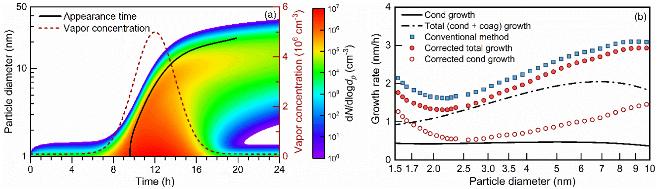
Figure 6 The appearance time method under a varying vapor concentration. The test condition is summarized in Table A1, No. 8. (a) An NPF event simulated using a discrete-sectional aerosol dynamic model. The vapor concentration is assumed to follow a normal distribution (with a background value of 10^5 \text{ cm}^{-3} ). The 100-nm background particles are not shown. The particle diameter as a function of the appearance time is shown in the solid line. (b) The theoretical and retrieved particle growth rates. Cond and coag are short for condensation and coagulation, respectively.
