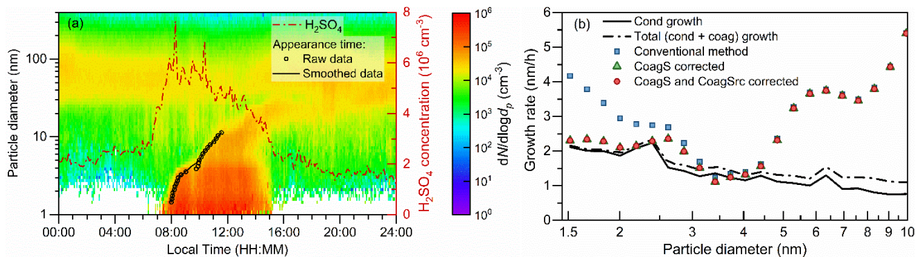
Figure 7 A case study for the appearance time method in the real atmosphere. (a) Aerosol size distribution and \text{H}_2\text{SO}_4 concentration measured on an NPF day. The event was measured on Feb. 24 th , 2018, in urban Beijing. (b) Measured growth rates using the conventional and corrected appearance time methods and the theoretical growth rate contributed by sulfuric acid condensation and particle coagulation. Cond and coag are short for condensation and coagulation, respectively. Note that the theoretical growth rate considers only the sulfuric acid condensation, hence, it may underestimate the overall condensation growth rate contributed by multiple condensing vapors.
