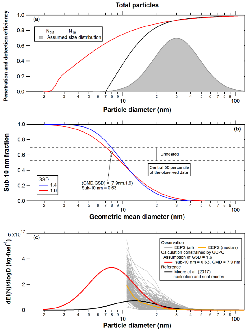
840 Figure 9: (a) Overall penetration and detection efficiencies for the unheated N_{2.5} and N_{10} . The shaded area represents an example of the 845 assumed particle number size distributions for calculating the number fraction of sub-10 nm particles. (b) Number fraction of sub-10 nm particles ( 1 - \Delta N_{10}/\Delta N_{2.5} ) obtained by convolution of the penetration and detection efficiency curves in (a) and assumed particle number size distributions having various GMDs and GSDs. The horizontal dashed lines indicate the central 50 percentile range (between 25 and 75 percentiles) of the observed data for the unheated mode. (c) Example of the particle number EI size distributions that explains the observed medians of the \Delta N_{10}/\Delta N_{2.5} ratios and EI( N_{2.5} ) for the unheated mode (red). The number EI size distributions with (\text{GMD, GSD}) = (12.7 \text{ nm}, 1.56) and (61 \text{ nm}, 1.48) , which correspond to the average nucleation and soot mode distributions (black) reported by Moore et al. (2017a), are shown for comparison. The size distributions of particle number EIs for the take-off plumes derived from the EEPS data (Fig. 8a) are also shown.
