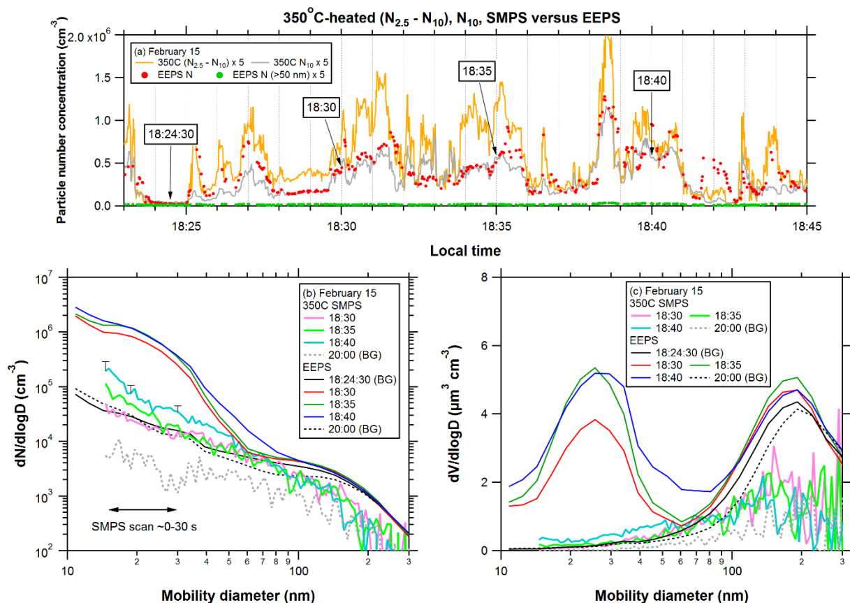
820 Figure 7: (a) Time series of 350°C heated N_{2.5} - N_{10} (orange), N_{10} (gray), total particle number concentrations derived from the EEPS data (EEPS N, red), and particle number concentrations for a diameter range of >50 nm measured by the EEPS (EEPS N (>50 nm), green) 825 obtained at 18:23–18:45 LT on February 15, 2018. The 350°C heated N_{2.5} - N_{10} , N_{10} , and EEPS N (>50 nm) data are multiplied by a factor of 5 for clarity. (b) Particle number size distributions measured simultaneously by the EEPS and 350°C heated SMPS for selected time periods indicated in (a). The average method for the EEPS is the same as that used in Fig. 6b. “BG” denotes a time period without enhancements of the aerosols and CO 2 . The upper ends of the error bars indicate the particle number concentrations incorporating the penetration efficiencies of particles through the sampling tubes and evaporation tube (Figs. 3 and S1). (c) Same as (b) but for the particle volume size distributions.
