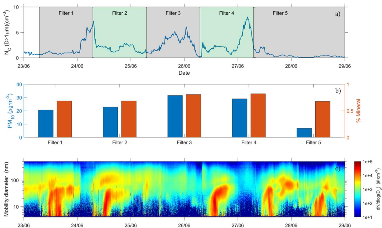
5 Figure 8. Temporal evolution of (a) coarse mode aerosol number concentration, (b) PM_{10} concentration and mineral matter fraction (%) and (c) aerosol size distribution from 23 to 29 June at SNS station.
