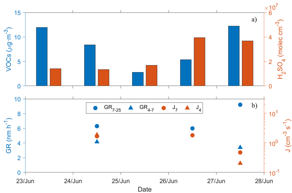
Figure 9. (a) VOCs and \text{H}_2\text{SO}_4 concentration and (b) GR and J in different size ranges from 23 to 28 June observed at SNS station.
