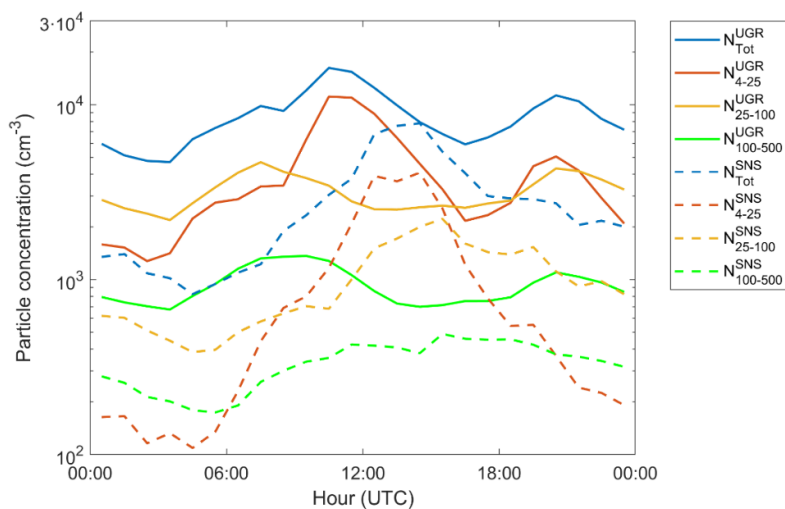
5 Figure 2. The mean diurnal variation of particle concentrations in different size ranges at SNS and UGR for the whole analysed period.
