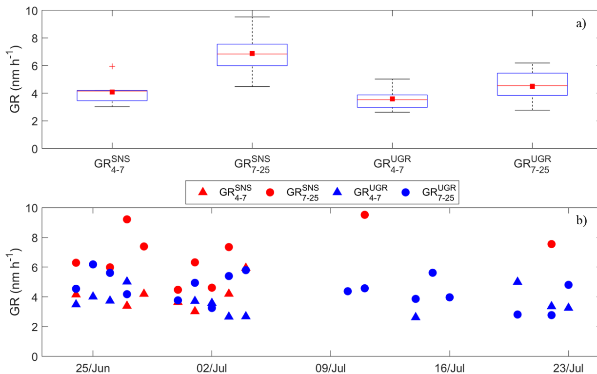
Figure 4. (a) Box and whisker plot of growth rates recorded at SNS and UGR stations. The red line represents the median of the data, the square represents the mean of the data and the lower and upper edges of the box represent 25th and 75th percentiles of the data, respectively. The length of the whiskers represents 1.5 \times interquartile range which includes 99.3% of the data. (b) Growth rates time series at SNS and UGR station.
