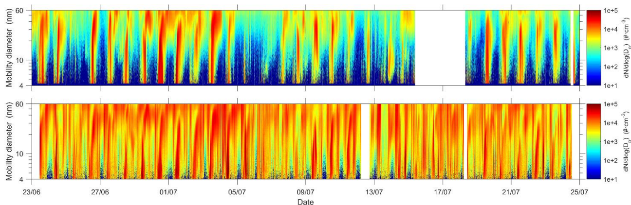
Figure 3. Size distribution time evolution from 23 June to 24 July at SNS (top) and UGR (bottom) station.
