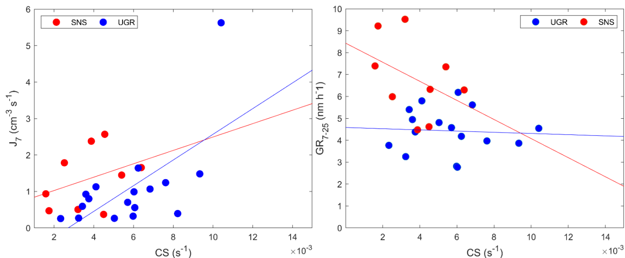
Figure 7. Relationship between CS (time window: 9:00-16:00 UTC) and J_7 (left) and GR_{7-25} (right) during study period.
