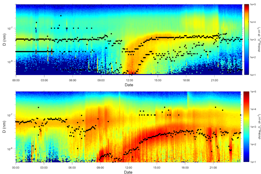
Figure S2. An example illustrating a case where (a) two aerosol modes appears at same time at SNS site and (b) local and regional event take place at UGR site.
