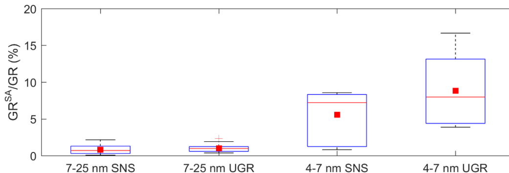
Figure 6. Box and whisker plot of sulfuric acid contribution to the total measured growth rate at SNS and UGR. The red line represents the median of the data, the square represents the mean of the data and the lower and upper edges of the box represent 25th and 75th percentiles of the data, respectively. The length of the whiskers represents 1.5 \times interquartile range which includes 99.3% of the data.
