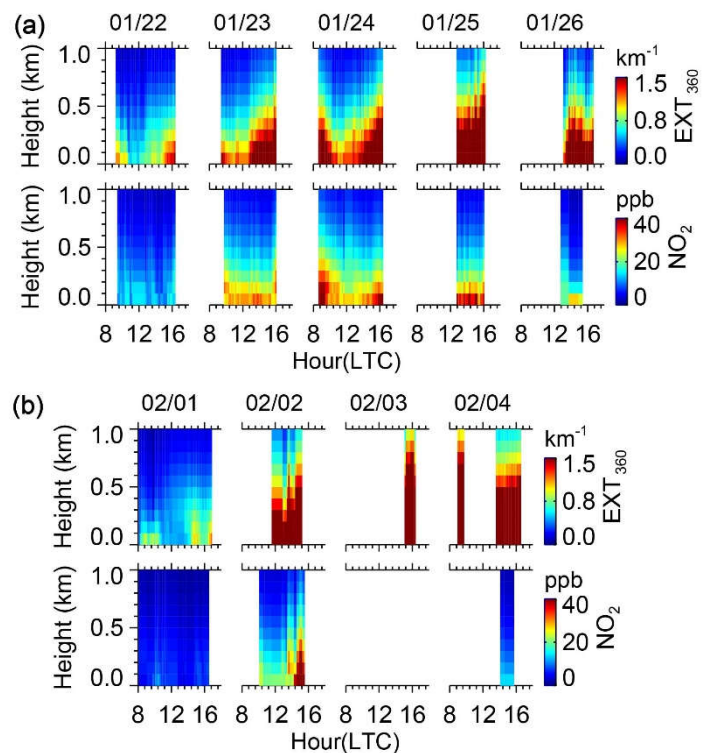
Figure 4. Curtain plots of MAX-DOAS observations. (a) \text{EXT}_{360} and \text{NO}_2 VMR from 22 to 26 Jan 2017, (b) \text{EXT}_{360} and \text{NO}_2 VMR from 1 to 4 Feb 2017.
