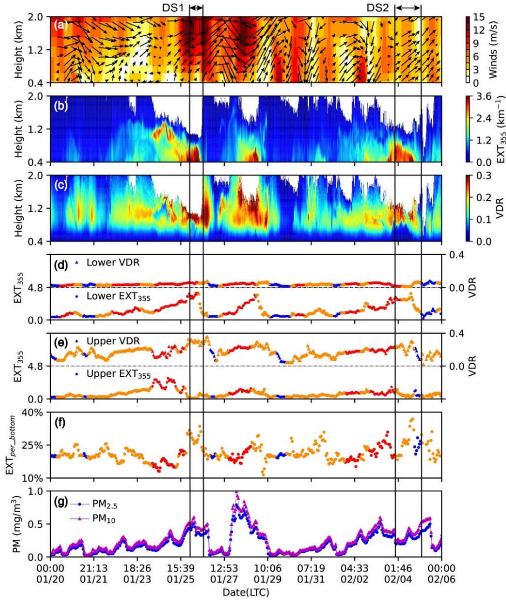
Figure 3. Periodic air pollution cycles in North China. The color contours show the vertical structure of (a) Horizontal winds simulated by WRF-Chem, (b) EXT_{355} and (c) VDR measured by RL. Temporal evolutions of spatially average VDR and EXT_{355} at (d) 450 m–550 m and (e) 950 m–1,050 m. (f) The percentage of bottom EXT_{355} . (g) Temporal evolutions of surface average PM_{2.5} and PM_{10} mass concentrations. The black arrow in (a) indicates the wind direction, upper arrow for south winds. The colors in (c) and (d) represent the air masses originating from southwest (red), Gobi desert (yellow), and sparsely populated northern mountain areas (blue), similar to those in Fig. 1. The observed PM_{2.5} and PM_{10} mass concentrations are the averages of the six environmental monitoring stations in Baoding. The percentage of bottom EXT_{355} is used to characterize the aerosol concentrations in the lower layer, which is defined as: EXT_{per\_bottom} = 100\% \times \sum_{z=400}^{600} EXT_{355}(z) / \sum_{z=400}^{1000} EXT_{355}(z) . Where EXT_{per\_bottom} is the percentage of bottom EXT_{355} , z is the height.
