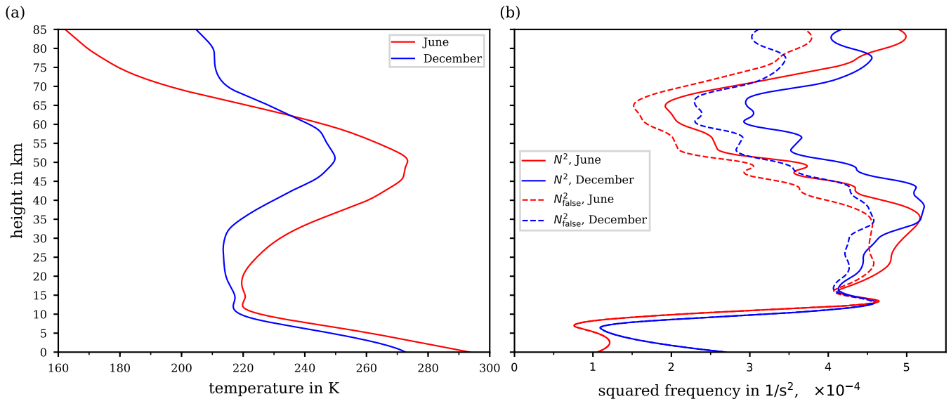
Figure 9. Vertical profiles of (a) the temperature up to 85 km altitude as typical for mid-latitudes in June (red curve) and December (blue curve). (b) Resulting wrong Brunt-Väisälä frequency N^2_{\text{false}} (dashed lines) and the true Brunt-Väisälä frequency N^2 (solid lines) for the two temperature profiles from panel (a).
