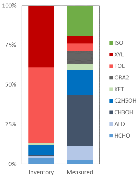
695 Figure 11. The percentage contribution of the MEIC VOC groupings to the total emission.
