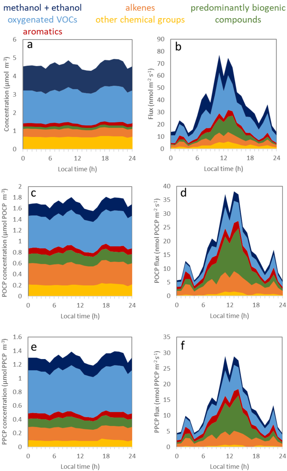
535 Figure 6. Total observed VOC concentration (a) and flux (b) measured during the summer field campaign, scaled using photochemical ozone creation potentials (POCPs) (c, d) and photochemical PAN creation potentials (PPCPs) (e, f).
