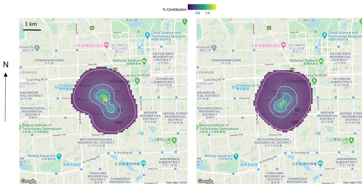
Figure 4. The campaign mean flux footprint climatologies for the winter (left) and summer (right) field campaigns. The IAP meteorological tower is represented by the red dot and surrounding 100 × 100 m cells are coloured by their mean contribution to the flux. The contour lines correspond to the distances from the tower where the surface contributions to the measured fluxes cumulate to 30, 60 and 90% respectively. Map tile sets are © Google.
