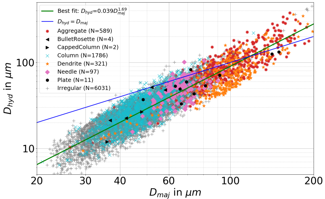
Figure 7. Relation between the hydrodynamic diameter D_{hyd} calculated using Eq. (7) and the measured particle size D_{maj} of falling crystals. Different crystal habits (classified by the trained predictor) are marked as different symbols and colors. Power law fit as green line, D_{hyd} = 0.039D_{maj}^{1.69} , with both D_{hyd} and D_{maj} in \mu m . The blue line represents D_{hyd} = D_{maj} .
