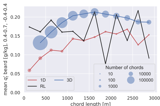
Figure 11. Mean water vapor anomalies below chord base as a function of chord length. The area over which the vertical velocity is averaged is marked by the grey box in figure 10. The size of the markers represents the number of chords in that 250 m bin. Note that there is no 3D value for chords below 250 m as we only compute scenes for chords with at least 10 data points as explained in section 2.
