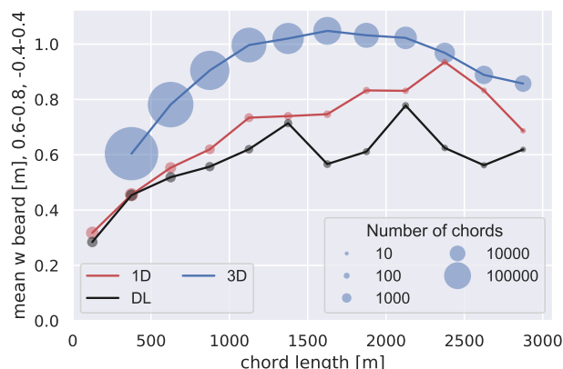
Figure 8. Mean regularized vertical velocity below chord base as a function of chord length. The area over which the vertical velocity is averaged is marked by the grey box in figure 9. The size of the markers represents the number of chords in that 250 m bin. Note that there is no 3D value for chords below 250 m as we only compute scenes for chords with at least 10 data points as explained in section 2.
