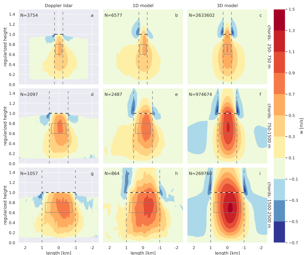
Figure 9. Regularized vertical velocity scenes from Doppler lidar observations (a,d,g), from 1D columns output (b,e,h), and from 3D snapshot (c,f,i). Chords were binned by lengths of 250-750 m (a,b,c), 750-1500 m (d,e,f), and 1500-2500 m (g,h,i). The black dashed and white horizontal line marks the chord base, the dashed grey lines the chord beginning and end, and the grey box area the area averaged for figure 8. See section 2.1 for information on the Doppler data, and sections 3.2 and 3.1 for descriptions of how chords were derived from the MicroHH simulations. Doppler lidar scenes are only shown where at least 70 % of the scenes contain data.
