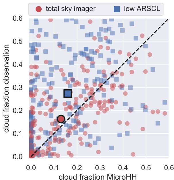
Figure 2. Cloud fraction of MicroHH simulations against two sets of cloud fraction measurements provided by the LASSO bundle browser of all used simulations. The total sky imager detects cloud fraction from a fish eye image of the sky, while the low ARSCL is a value added produce in which cloud fractional occurrence is determined for 15-minute windows. Observations are only included when the cloud fraction is below 0.6, to reduce contamination of non convective clouds, and observations are only used when the quality flags are ideal. The mean of each product is marked by the large symbol with the black border. The mean model values differ due to the differing time availability of observations.
