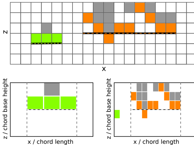
Figure 3. Illustration of chords, chord base height, and scenes as defined in section 3. The top half shows a sketch of a z - x slice of 3D output. The filled in grid boxes are cloudy cells. The green and orange cells show the cloudy cells which would be detected as two chords from the surface. The thick black lines mark the chord length and the chord base height of the two chords. The two lower boxes show the resulting 2D scenes after normalizing the two chords with their respective chord base height and length. For an example using Doppler lidar data see Lareau et al. (2018, Figure 1).
