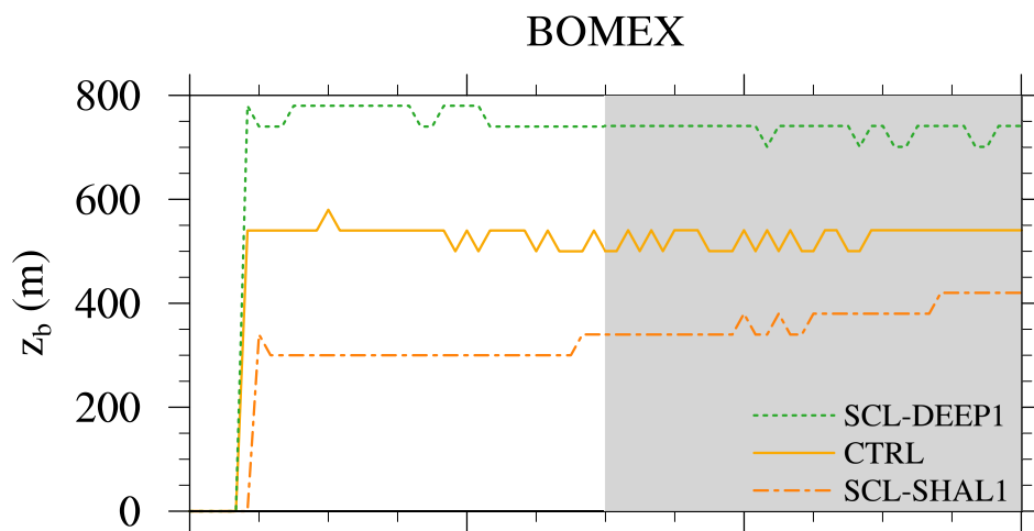
Fig. 7. Cloud-base height for the subcloud-layer depth experiments.
