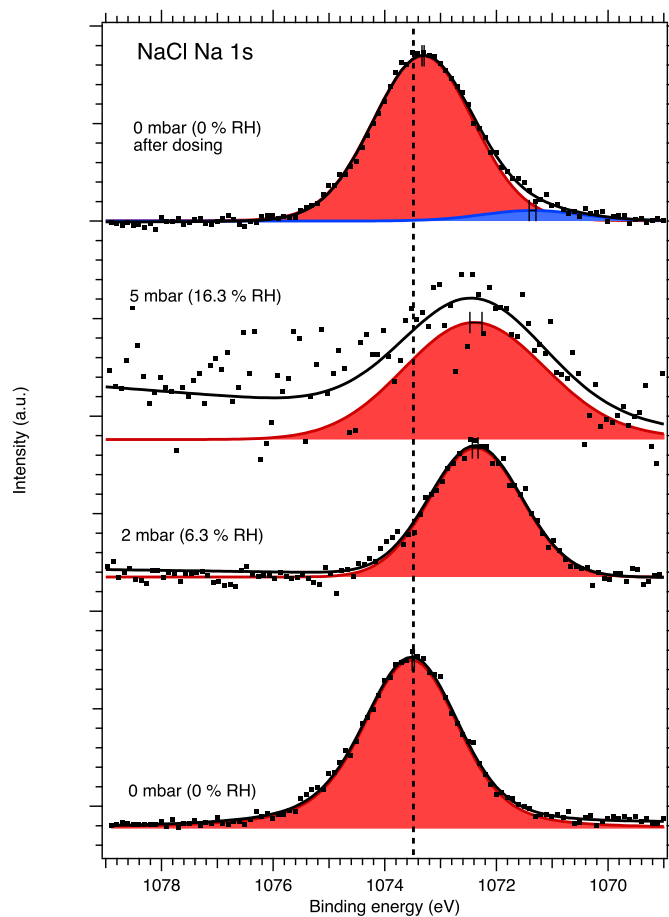
Figure 1. Na 1s XPS spectra of NaCl aerosol particles recorded at different water vapor pressures (relative humidities, RH). The dots-point markers show the recorded data and the solid lines the fit envelope curve and the . The spectra are fit using a single, symmetric Voigt peak shown in red and with an additional peak in blue peaks necessary to explain the fitted Voigt profiles spectrum at 0 mbar after water exposure. The dashed vertical line shows the binding energy of Na 1s at 0 mbar pressure (0 % RH) at the beginning of the experiments. Error bars show the estimated uncertainty in the peak position from Monte Carlo analysis. Photon energy was 1486.6 eV from the Al anode.
