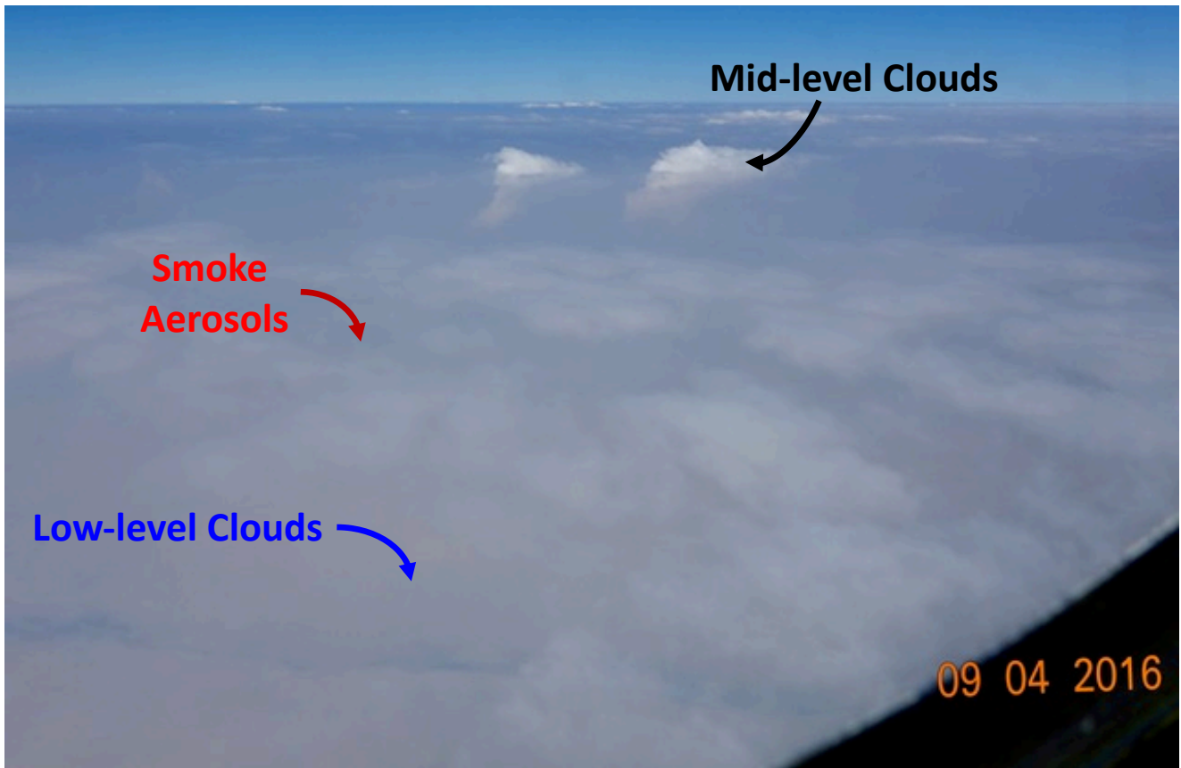
790 Figure 1: An Image taken during the NASA ORACLES Field campaign on September 4, 2016, showing mid-level clouds and smoke above the low-level clouds. Image taken by Paquita Zuidema.
