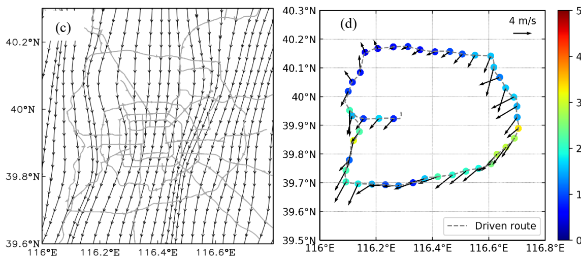
Fig. 8 Average wind stream and NO 2 VCD ( 10^{16} molecules \text{cm}^{-2} ) distributions under the two different types of wind field over Beijing: (a) south wind, (b) NO 2 VCD under south wind, (c) north wind, and (d) NO 2 VCD under north wind.
