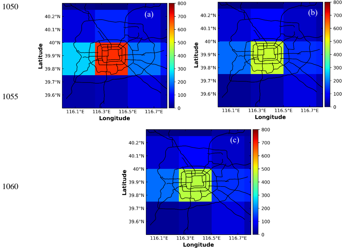
1050 1055 1060 1065 Fig. 10 Spatial distributions of monthly averaged NO x emissions rate (mole km -2 h -1 ) over Beijing based on the MEIC inventory in (a) January, (b) September, and (c) October in 2012.
