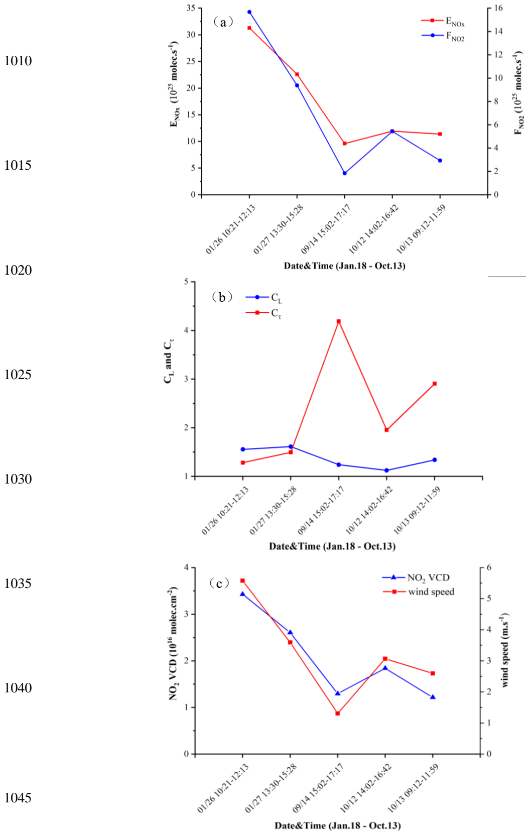
Fig. 9 Journey-to-journey variations in (a) F_{NO_2} and E_{NO_x} , (b) c_\tau and c_L , (c) NO_2 VCD and mean wind speed for five circling journeys on the 6th Ring Rd of Beijing in January, September, and October, 2014.
