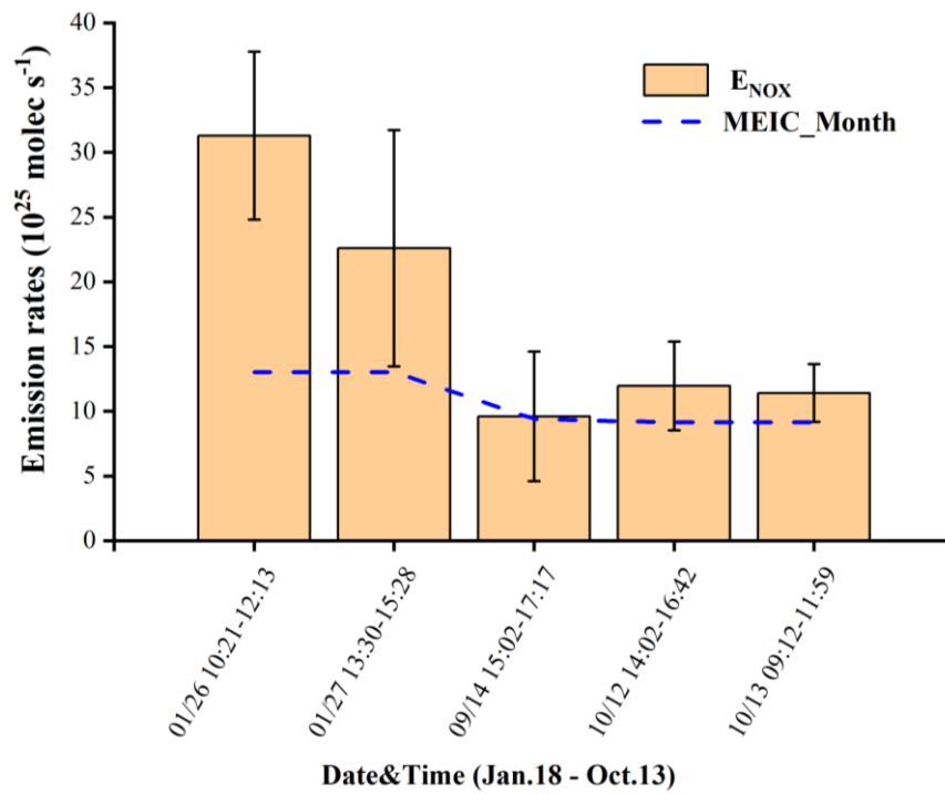
Fig. 11 Journey-to-journey variations in estimated E_{NO_x} and corresponding monthly emissions rate from the MEIC inventory (MEIC_Month) within the 6th Ring Rd of Beijing in January, September, and October 2014. Error bars represent the uncertainties in estimated E_{NO_x}
