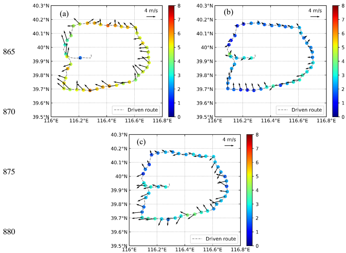
Fig. 5 Distributions of monthly averaged NO 2 VCD ( 10^{16} molecules \text{cm}^{-2} ) on the 6th Ring Rd of Beijing in (a) January, (b) September, and (c) October, 2014.
