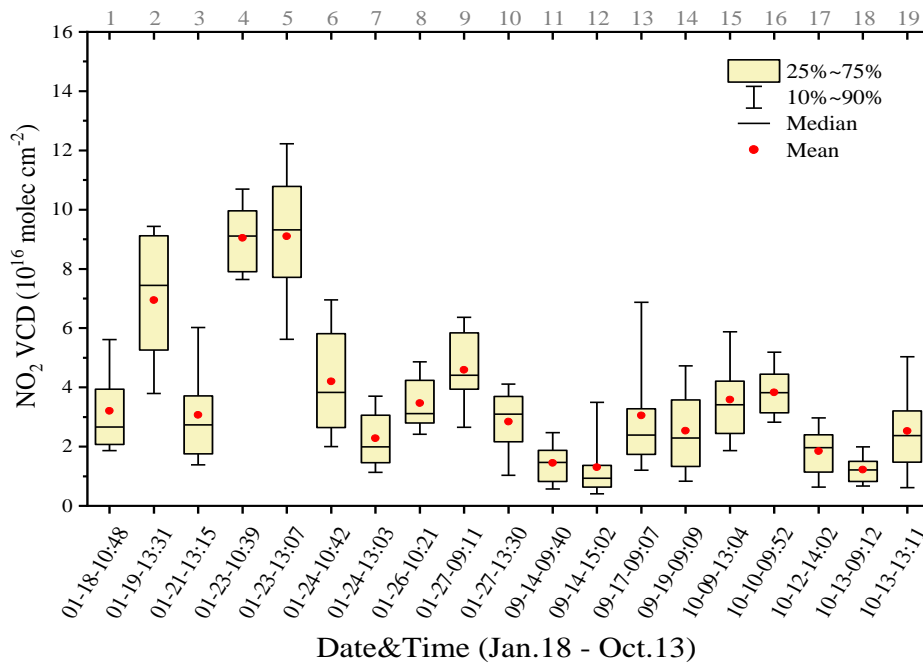
835 Fig. 4 Time series of the tropospheric NO 2 vertical column density (VCD) for 19 circling journeys on the Sixth Ring Road of Beijing in January, September, and October, 2014. Lower (upper) error bars and yellow boxes are the 10th (90th) and 25th (75th) percentiles of the data of each journey, respectively. Hyphens inside the boxes are the medians, and red circles are the mean values. The numbers of each journey are labeled at the top axis. See Table 1 for detailed information about each journey.
