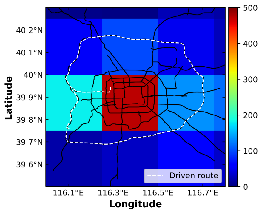
775 Fig. 1 Driving routes (white dash line) of the Car MAX-DOAS experiment on the 6th Ring Rd of Beijing and distribution of yearly averaged NO x emission rate (mole km -2 h -1 ) from the MEIC for the year 2012.
