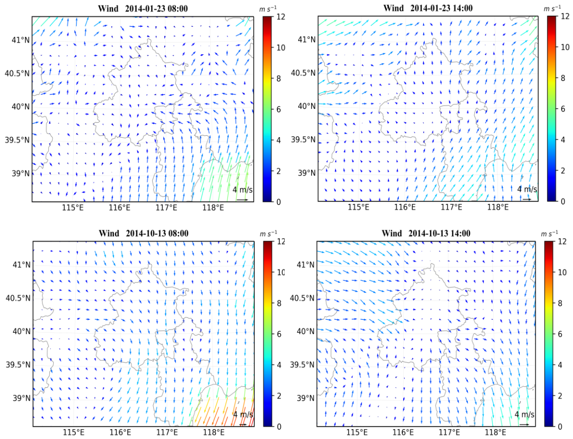
945 Fig. 7 Wind fields in Beijing and the surrounding area from ECWRF at 08:00 (left column) and 14:00 (right column) BJT on January 23 and October 13, 2014.
