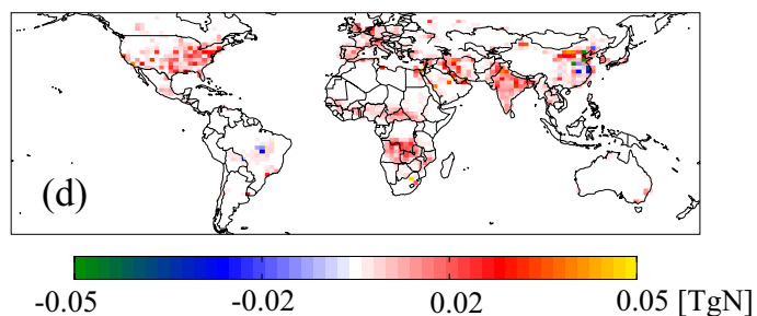
740 Figure 1. (a) Global total NO x emissions from the bottom-up inventory and the differences between 4D-Var posterior and bottom-up estimates constrained by (b) NASA standard product v3, (c) DOMINO product v2, and (d) QA4ECV product in 2010.
