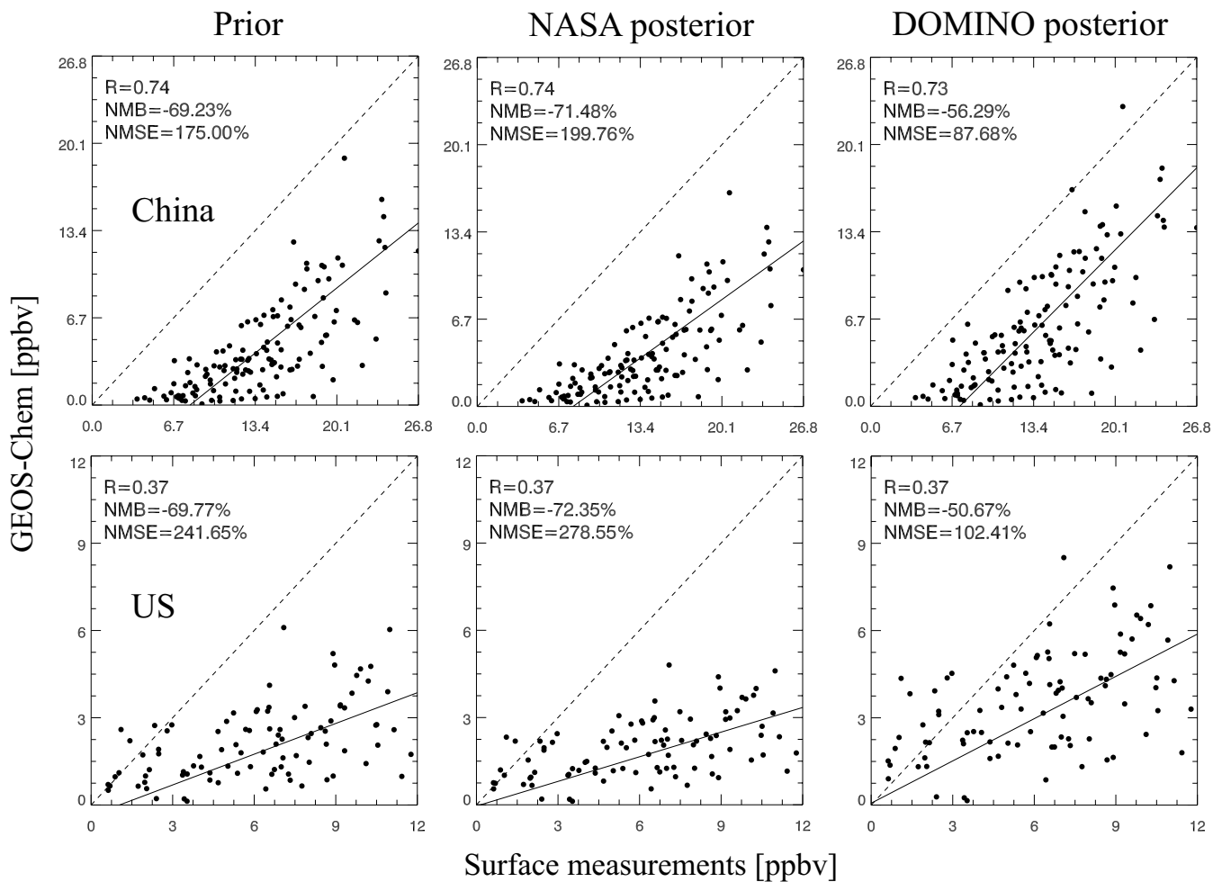
Figure 2. Evaluation of annual mean surface NO 2 mixing ratios with measurements in China (top) and the US (bottom) in 2015.
