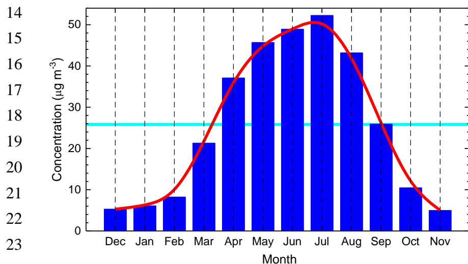
25 Figure S1. Overall distribution of monthly median O 3 concentrations averaged over the whole measurement 26 interval. The horizontal line in cyan indicates the overall annual mean concentration of 26 µg m -3 , and the smooth 27 curve in red serves to guide the eye.
