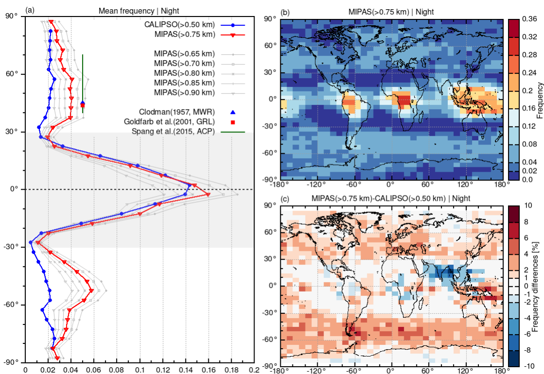
Figure 6. Zonal mean CTH occurrence frequencies (a) and geospatial distribution on a 5^\circ \times 10^\circ latitude-longitude grid (b) of 6-year mean nighttime occurrence frequencies of stratospheric cirrus clouds observed by MIPAS (CTHs >0.75 km above tropopause). c) Difference between MIPAS and CALIPSO (CTHs >0.50 km above tropopause) occurrence frequencies.
