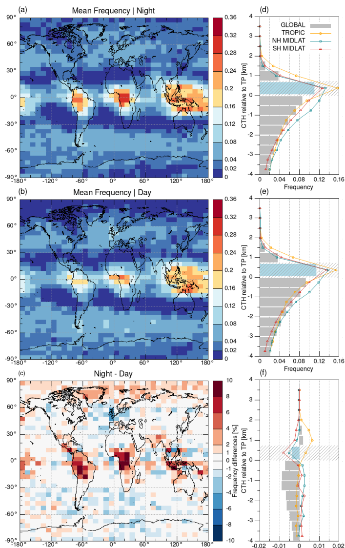
Figure 8. Nighttime (a) and daytime (b) CTH occurrence frequencies of stratospheric cirrus clouds derived from June 2006 to April 2012 MIPAS measurements. (c) Difference between MIPAS nighttime and daytime occurrence frequencies. (d), (e), (f) show the corresponding global mean frequencies of CTHs relative to the tropopause for nighttime, daytime, and their difference, respectively. The MIPAS tropopause threshold from 0 to 0.75 km above the tropopause is marked gray.
