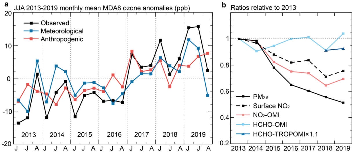
Figure 6. Trends in summertime ozone and related anthropogenic drivers in the North China Plain (NCP). The left panel (a) shows time series of monthly mean MDA8 ozone (ppb) anomalies averaged over the MEE sites relative to the 2013–2019 summer (JJA) mean. Values are shown as anomalies for individual JJA months (3 points per year). Observed trends are compared to the meteorologically driven trends diagnosed by the MLR model, and to the residuals determining the anthropogenically driven trend. The right panel (b) shows time series of observed JJA mean quantities averaged over the NCP: PM 2.5 (black, solid) and NO 2 (black, dashed) concentrations from the MEE sites, tropospheric NO 2 (blue, solid) and HCHO (pink, solid) column densities from the OMI satellite instrument, and HCHO column density from the TROPOMI satellite instrument (dark blue, solid). Values are presented as ratios relative to 2013. The TROPOMI HCHO data for 2018 have been scaled to the OMI data for that year with the multiplicative factor indicated in legend.
