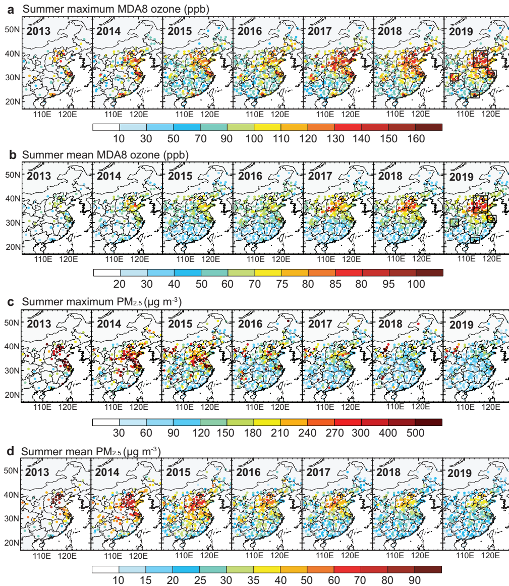
Figure 1. Summer (JJA) concentrations of maximum MDA8 ozone (a), mean MDA8 ozone (b), maximum PM_{2.5} (c), and mean PM_{2.5} (d) for 2013–2019 at the network operated by the China Ministry of Ecology and Environment (MEE). Rectangles denote the four megacity clusters discussed in the text: North China Plain (NCP; 34°–41°N, 113°–119°E), 5 Yangtze River Delta (YRD, 30°–33°N, 119°–122°E), Pearl River Delta (PRD, 21.5°–24°N, 112°–115.5°E), and Sichuan Basin (SCB, 28.5°–31.5°N, 103.5°–107°E).
