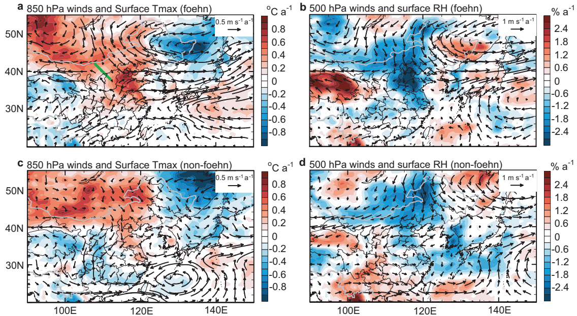
Figure 5. June mean trends in meteorological variables over 2013–2019 under foehn (top) and non-foehn (bottom) conditions (a) Trends in 850 hPa winds ( \text{m s}^{-1} \text{a}^{-1} ) and surface daily maximum temperature ( ^{\circ}\text{C a}^{-1} , shaded) under foehn conditions; (b) Trends in 500 hPa winds ( \text{m s}^{-1} \text{a}^{-1} ) and surface relative humidity ( \% \text{a}^{-1} , shaded) under foehn conditions; (c, d) are the same as (a, b) but for non-foehn conditions. Data are from the MERRA-2 re-analysis and trends are obtained by ordinary linear regression. Foehn conditions are diagnosed by a foehn index defined by the 850 hPa northwesterly wind averaged along a section from ( 42^{\circ}\text{N} , 108^{\circ}\text{E} ) to ( 38^{\circ}\text{N} , 112^{\circ}\text{E} ) (green line in a ). The days with positive (negative) foehn index are taken as foehn (no-foehn) conditions. Meteorological data are from the MERRA-2 reanalysis.
