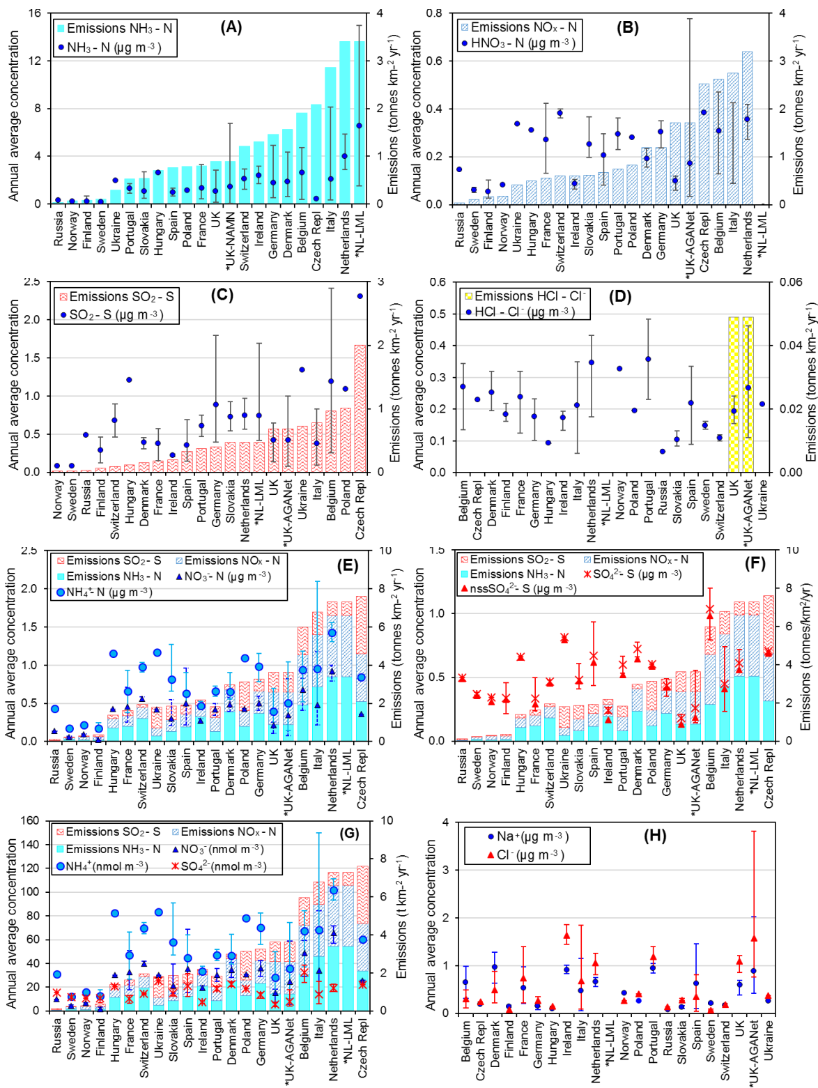
Figure 9: Comparisons of annual averaged gas and aerosol concentrations (2007–2010) of sites in the NEU DELTA® network, grouped by countries, with the respective 4-year averaged annual emission densities of gases ( \text{NH}_3 , \text{NO}_x and \text{SO}_2 ) over the same period. Monitoring data from 3 national monitoring networks: *UK NAMN ( \text{NH}_3 from 72 sites and \text{NH}_4^+ from 30 sites; Tang et al., 2018a), *UK AGANet (raw uncorrected \text{HNO}_3 , \text{SO}_2 , \text{HCl} , \text{NO}_3^- , \text{SO}_4^{2-} , \text{Cl}^- , \text{Na}^+ from 30 sites; Tang et al. 2018b) and *NL-LML ( \text{NH}_3 and \text{SO}_2 from 8 sites; van Zanten et al. 2017) are also included to illustrate the wider range of concentrations from larger numbers of sites. Error bars show the minimum and maximum concentrations measured in each country in the network. Where error bars are not visible, this indicates either that the country has measurement from just one site, or the range of concentrations measured are very close to the average.
