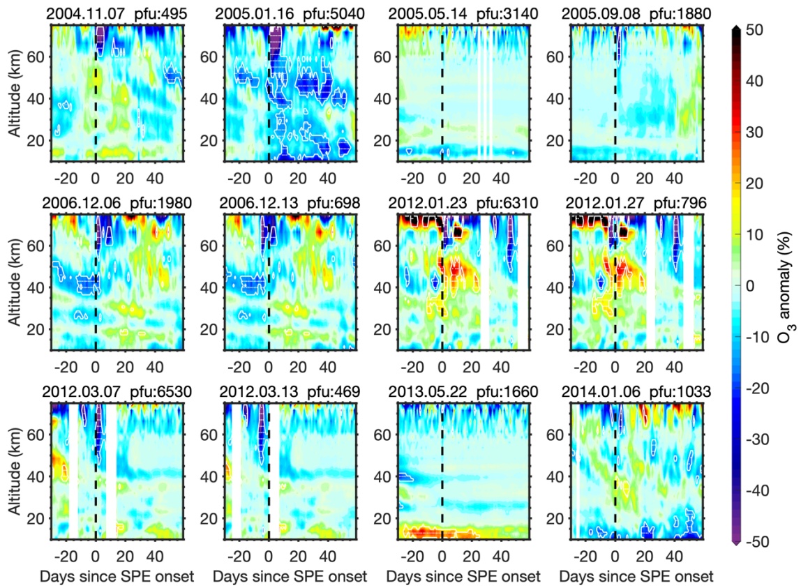
Figure S2. Same as Fig. S1 but the MLS ozone anomalies are calculated by subtracting a daily ozone climatology using median (instead of mean) values of MLS data from 2004 to date.
