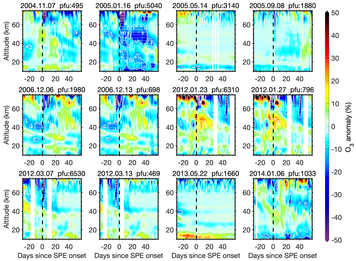
Figure S1. Same as Fig. 3 but the MLS ozone anomalies are reported as relative changes (%).
