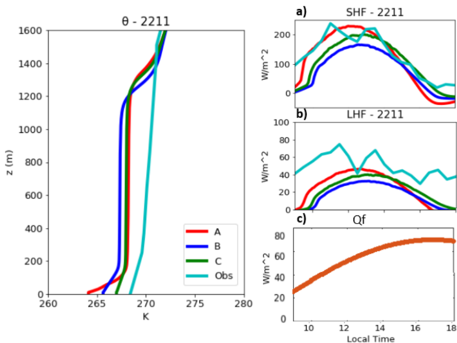
Figure 2. Potential temperature ( \theta ) profiles at 8 pm (left), a) Sensible Heat Flux (SHF) and b) Latent Heat Flux (LE) diurnal profiles (right) for no anthropogenic heat flux (A (Red) – C_h = 2 \times 10^6 ( J m^{-3} K^{-1} )), B (Blue) – C_h = 7 \times 10^6 ) and an anthropogenic heat flux (C (Green) – C_h = 7 \times 10^6 ) and observations. Where c) shows anthropogenic heat flux ( Q_f ) used in the simulation
