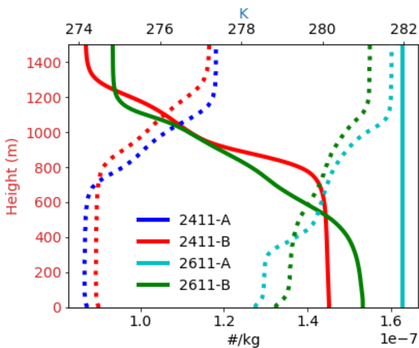
Figure 7. Number mixing ratio (solid) and potential temperature (dashed) vertical profiles at 5pm for constant vertical aerosol profiles on 24/11 (Blue) and 26/11 (Turquoise) and varied aerosol vertical profiles on 24/11 (Red) and 26/11 (Green)
