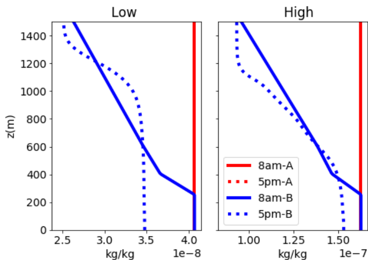
Figure 6. Aerosol mass mixing ratio vertical profiles for low and high aerosol loading simulations on 26/11, for constant aerosol profile (red) and vertically varying aerosol profiles (blue) at initial timestep (solid) and after 9 hours simulation (dashed)
