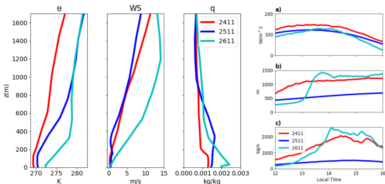
Figure 3. Left - Initial vertical profiles of Potential Temperature ( \theta ), Wind Speed (WS) and Total Water Mixing Ratio (q) and Right - a) Sensible Heat Flux, b) Height of maximum gradient in theta, c) Vertical integral of TKE for 24/11 (red), 25/11 (blue) and 26/11 (turquoise) for simulations with no aerosols (Case 1)
