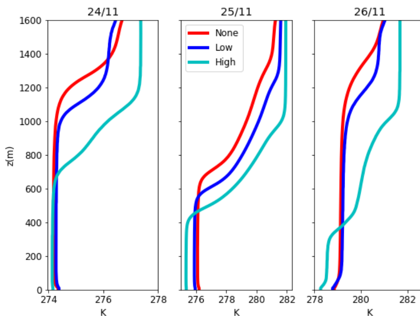
Figure 4. Potential temperature profiles at 5pm for 24/11, 25/11 and 26/11, with no aerosols (red), low aerosol loading (blue) and high aerosol loading (turquoise)
