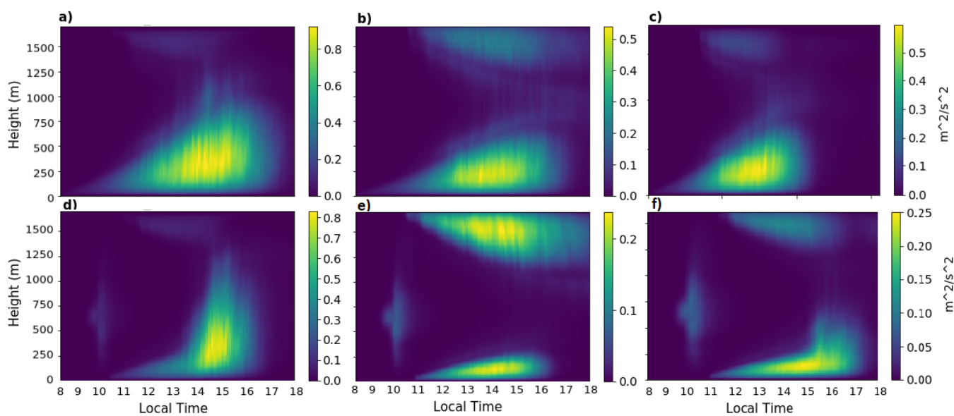
Figure 8. Variance in vertical velocity ( \sigma_w^2 ) for case 2 and case 3 simulations on 24/11 (a-c) and 26/11 (d-f) for low aerosol loading (a and d), high aerosol loading (b and e) and high loading with a varied aerosol vertical profile (c and f)
