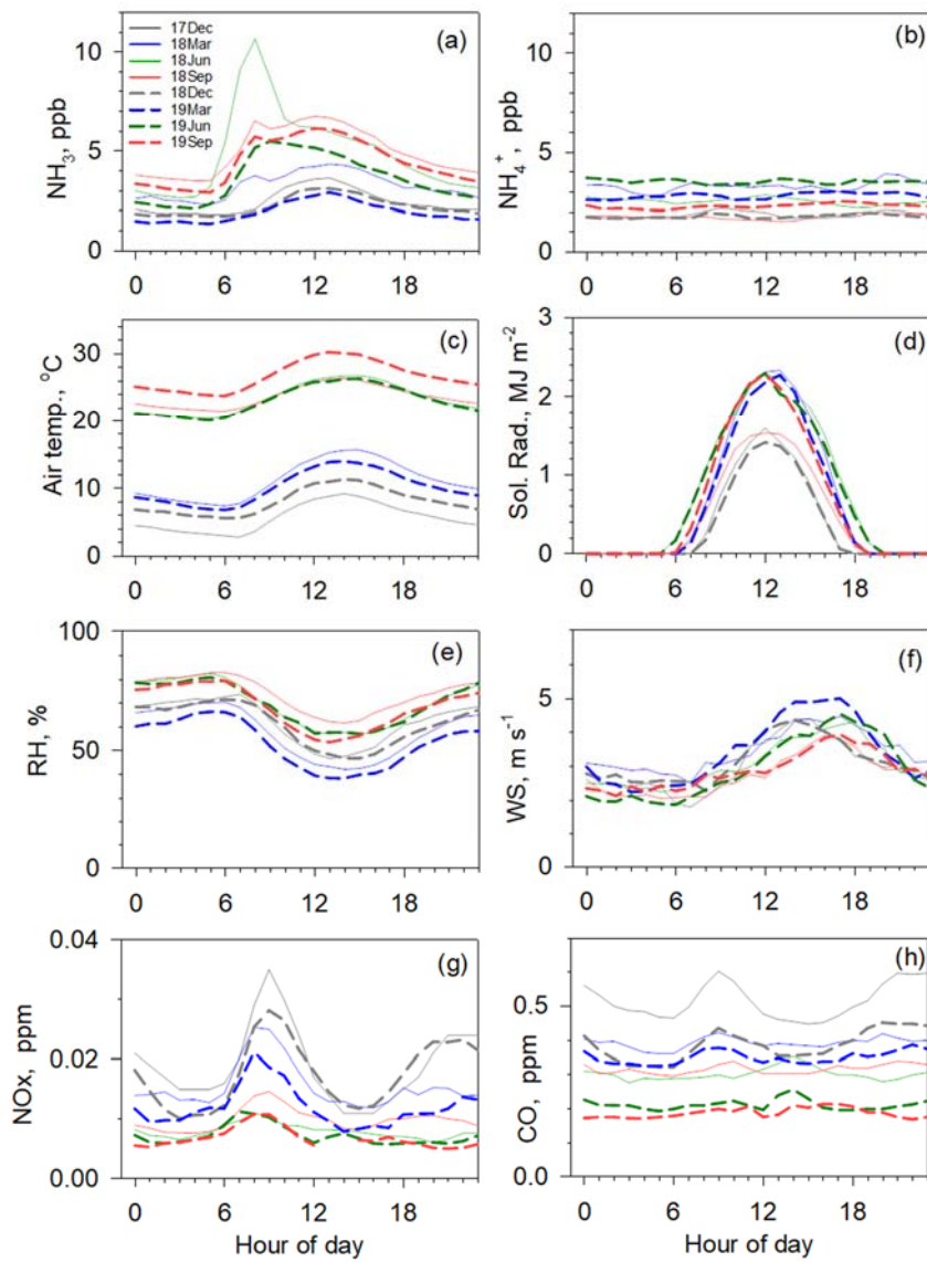
670 Figure 4 Hourly averages of various concentrations and meteorological parameters for several months: December (fine gray), 2017; March (fine blue), June (fine green), September (fine orange), and December (dotted gray), in 2018; March (dotted blue), June (dotted green), September (dotted orange), 2019; a) \text{NH}_3 , b) \text{NH}_4^+ , c) air temperature, d) solar radiation, e) relative humidity, f) wind speed, g) \text{NO}_x , h) CO.
