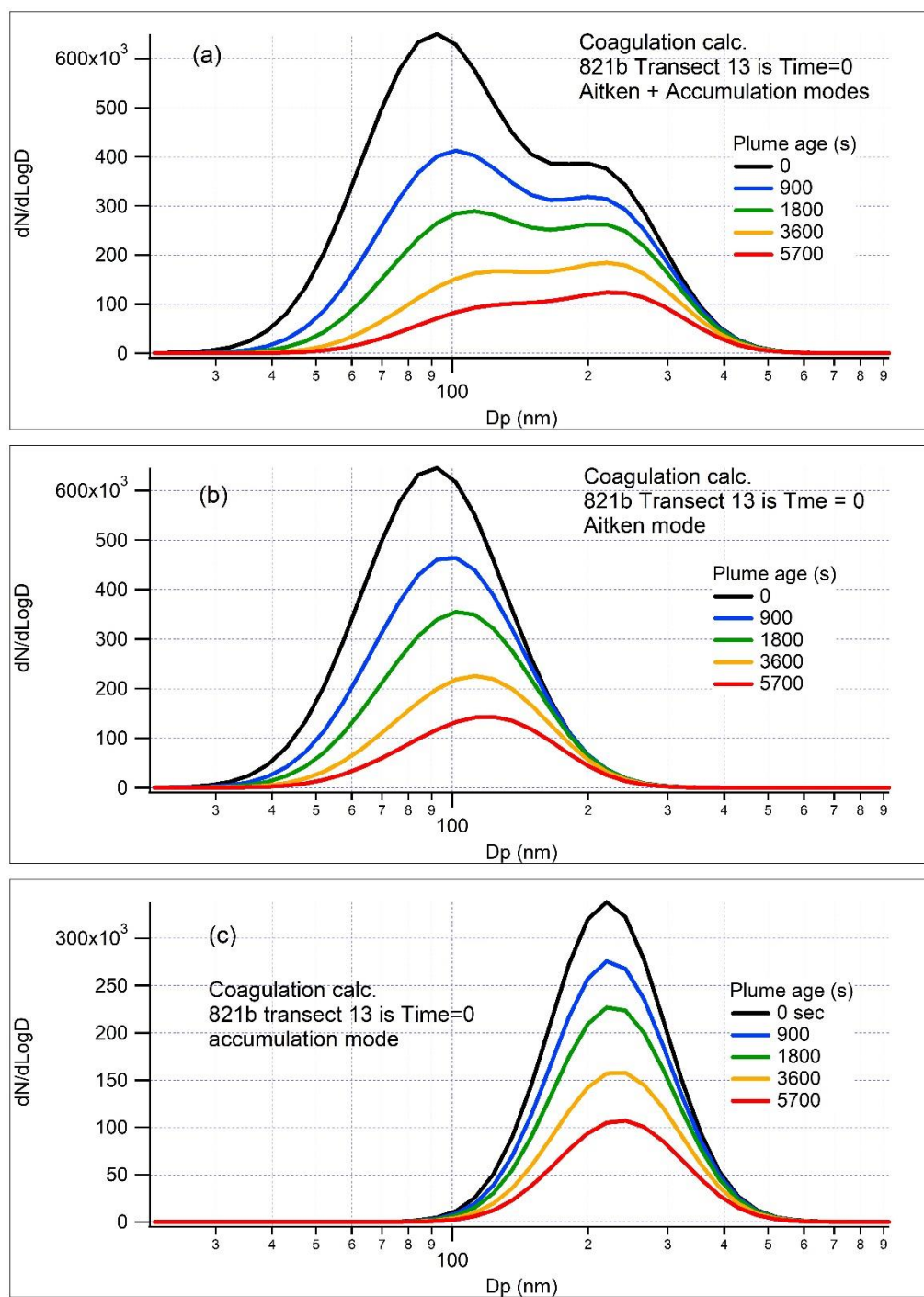
Figure 2. Time evolution due to coagulation of aerosol size distributions in Fig. 1 for (a) two modes, (b) Aitken mode, and (c) accumulation mode. Curves at 0, 900, 1800, 3600, and 5700 s, correspond to the initial conditions on transect 13 and the calculated size distributions for downwind transects 12, 11, 10, and 8 (see Fig. 19b of acpd submission)
