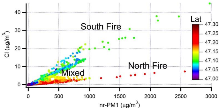
Figure 6. \text{Cl}^- concentration as a function of \text{nr-PM1} for flight 730b. Data points are at 1 Hz. Spatial locations of North and South fires shown in Fig 3.
