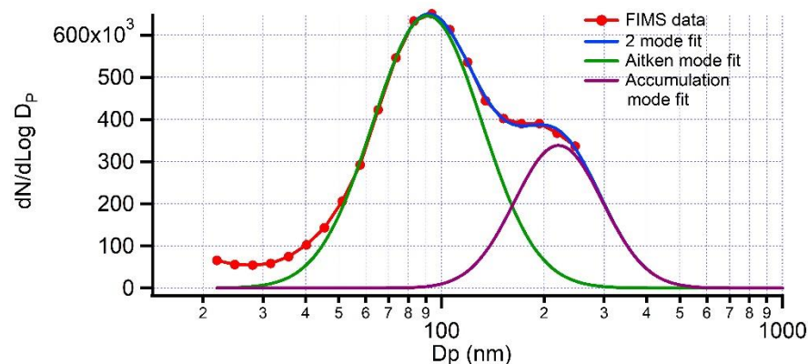
Fig 1. FIMS dN/d\log D_p averaged over transect 13, showing double log normal fit, and log normal fits to Aitken mode, and accumulation mode.
