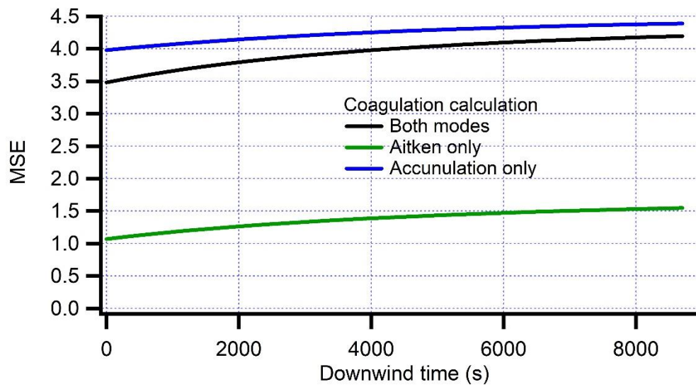
Figure 3. Time evolution of MSE. Transect 8 is 5700 s downwind of transect 13, the starting point for the coagulation calculation. A four-fold dilution occurs between time=0 and time=5700.
