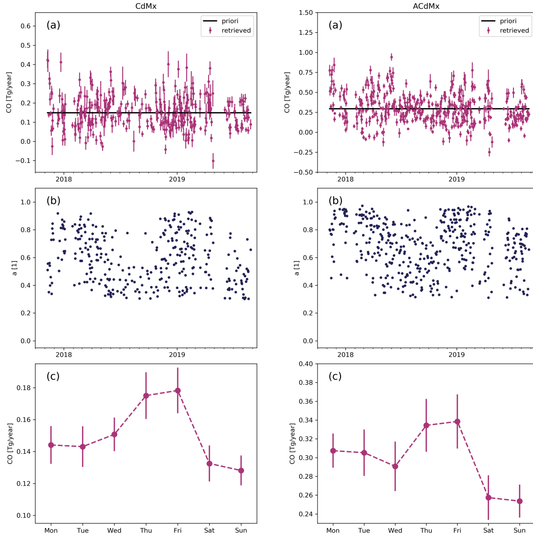
Figure 7. Retrieved CO Emissions from the TROPOMI data for the tracers CdMx (left panel) and ACdMx (right panel). (a) Time series of individual retrieved CO emissions. The error bars indicate the error of the fit and the black line is the time invariant priori used in the fit. (b) degree of freedom of the scaling factor for the tracer field. Only data with dofs > 0.3 is accounted for. (c) Weekly cycle of the CO emissions. Median values are shown and the error bars are the standard error of the mean deploying the delta percentile as a robust estimation of the standard deviation.
