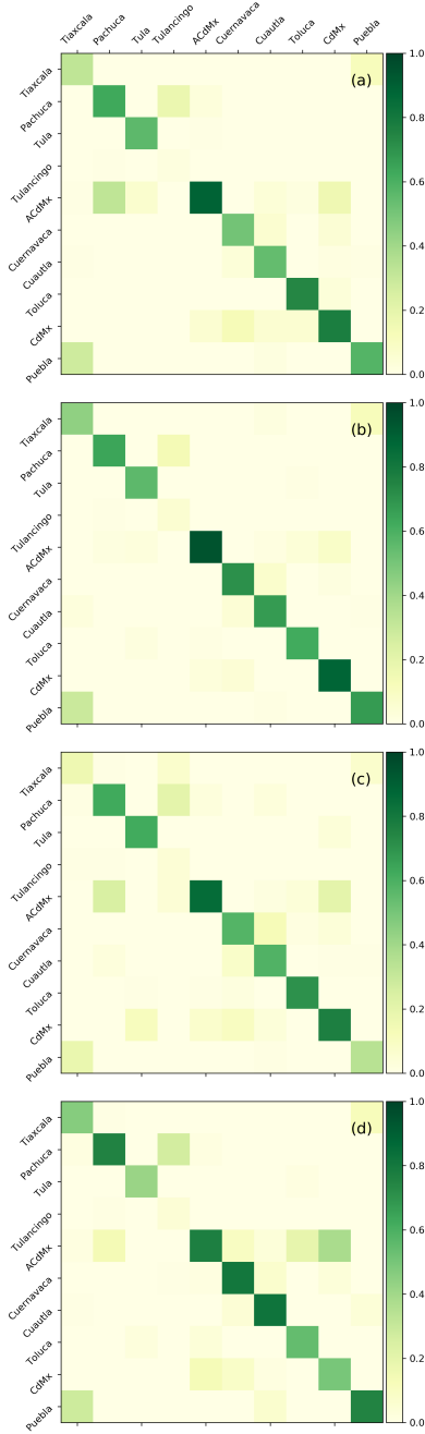
Figure 6. Averaging kernel matrices showing the sensitivity and cross-sensitivities for the scaling of the different tracer fields. The same cases as in Fig. 5 are shown for the dates (a) the 20th of September, (b) the 7th of November, (c) the 19th of November 2018 and (d) the 17th of August 2019 but deploying the regularized retrieval.
