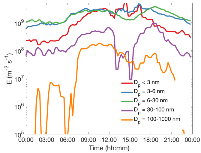
Figure A2. Average diurnal cycles of particle number emissions into different size ranges on non-NPF event days.
