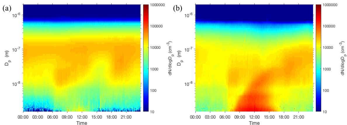
270 Figure 3: Average diurnal variation of particle number concentration size distributions (a) on days without NPF events and (b) on NPF event days.
