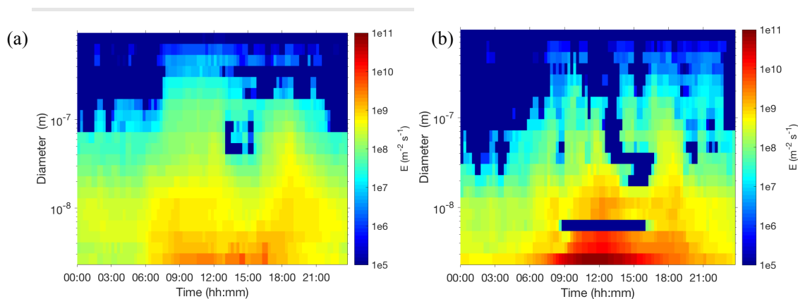
300 Figure 4: Average diurnal variation of particle number emission size distributions (a) on days without NPF events and (b) on NPF event days.
