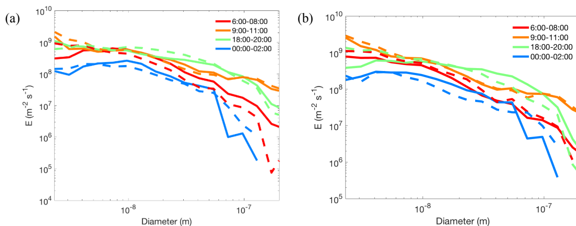
Figure A5: Average particle number emission size distributions for non-NPF event days (a) when wind is coming from the south-eastern directions ( 45^{\circ} – 225^{\circ} ; solid lines) and from the north-western directions ( 225^{\circ} – 45^{\circ} ; dashed lines), and (b) when wind speed is predominantly below 0.6 m/s (solid lines) and over 1.1 m/s (dashed lines).
