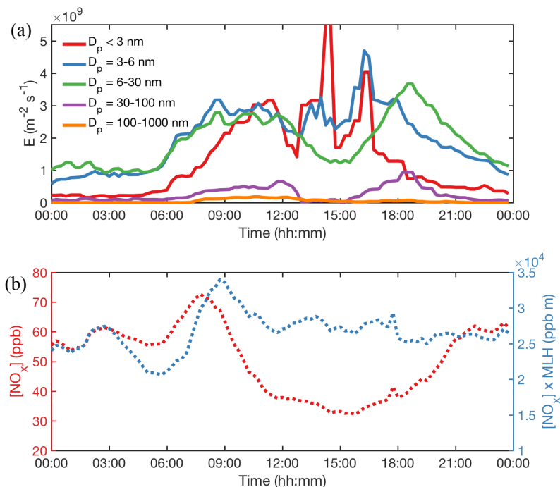
340 Figure 5: Average diurnal cycles of (a) particle number emissions into different size ranges on non-NPF event days, (b) the concentration of \text{NO}_x (nitrogen oxidizes) and its product with MLH (mixing layer height). For particle number emissions depicted in a logarithmic scale, see Fig. A2 in Appendix.
