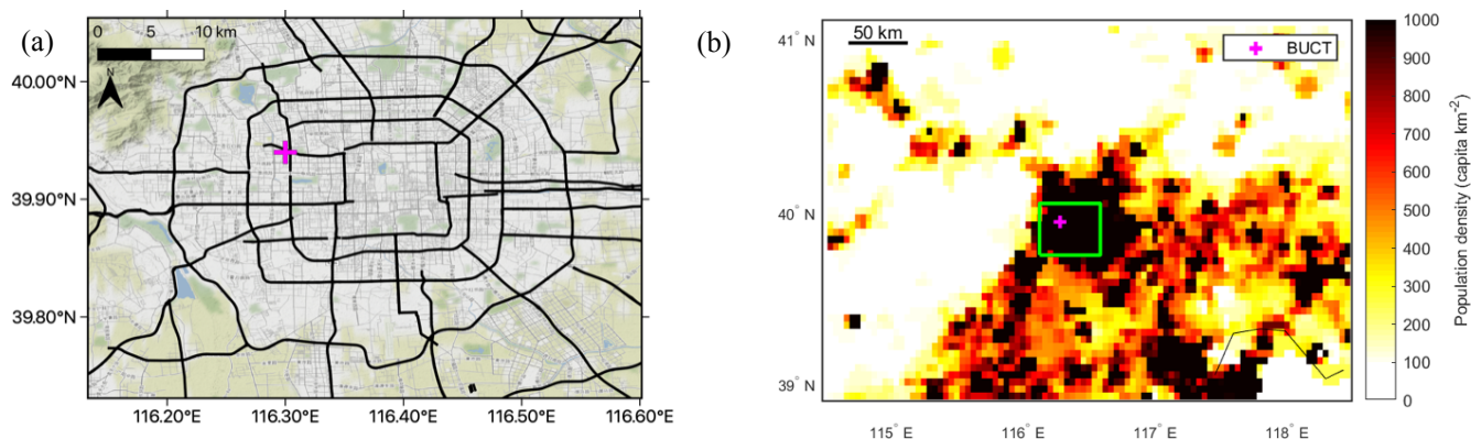
245 Figure 1. The maps of (a) urban Beijing and its main roads, and (b) the region around Beijing with the population density (year 2015) shown as color. The location of the measurement site of BUCT is shown with a magenta cross in both maps. The green rectangle in (b) corresponds to the region shown in (a). In (a) the map data obtained from Stamen Design (CC BY 3.0) and © OpenStreetMap contributors 2020. Distributed under a Creative Commons BY-SA License (ODbL). In (b) the population density data obtained from Gridded Population of the World (GPWv4.10; CC BY 4.0).
