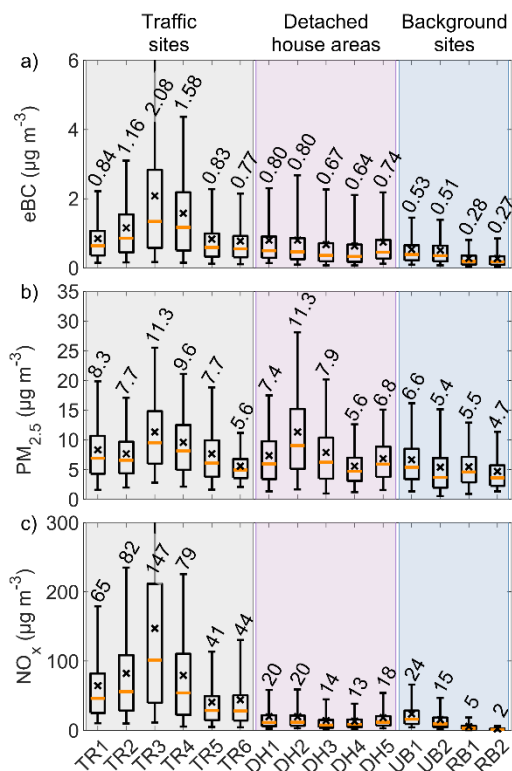
785 Figure 2: Statistics of the a) eBC, b) \text{PM}_{2.5} , and c) \text{NO}_x concentrations at each station. The boxplots are presented for 1 h mean values. The orange line in the middle of each box represents the median, the edges of the boxes represent the 25 th and 75 th percentiles, and the whiskers represent the 5 th and 95 th percentiles. The black cross is the arithmetic mean, and its numerical value is reported above each box. The background color represents the station type: gray for traffic sites (TR), purple for the detached housing sites (DH), and blue for the background sites (UB for urban and RB for regional background). The 75 th percentiles of the eBC and \text{NO}_x concentration at TR3, which are not visible at the figure, were 6.7 and 440 \mu\text{g m}^{-3} , respectively. 790
