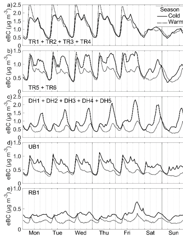
Figure 6: Diurnal variation of eBC for different station categories: a) traffic sites that were not influenced by wood burning (TR1–4), b) traffic sites that were influenced by wood burning (TR5–6), c) detached housing sites (DH1–5), d) urban background (UB1), and e) regional background (RB1). The diurnal variation is determined separately for the cold (from November to March) and warm (from May to September) periods.
