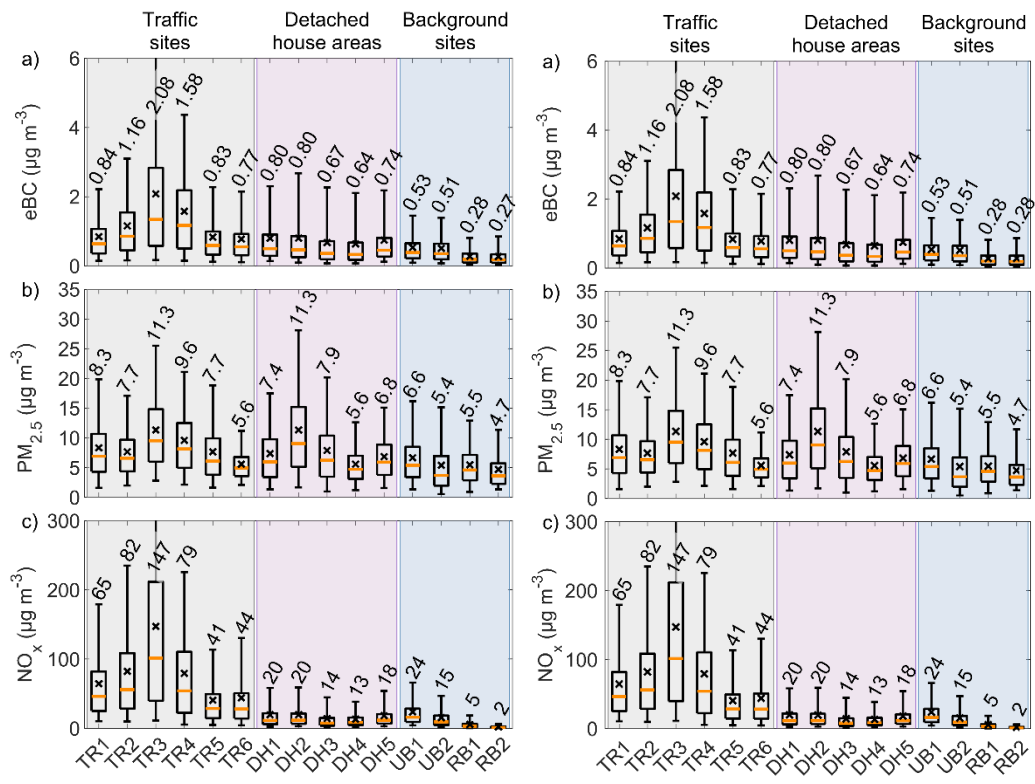
Figure 2: Statistics of the a) eBC, b) PM 2.5 , and c) NO x concentrations at each station. The boxplots are presented for 1 h mean values. The orange line in the middle of each box represents the median, the edges of the boxes represent the 25 th and 75 th percentiles, and the whiskers represent the 5 th and 95 th percentiles. The black cross is the arithmetic mean, and its numerical value is reported above or below each box. The background color represents the station type: gray for traffic sites (TR), purple for the detached housing sites (DH), and blue for the background sites (UB for urban and RB for regional background). The 75 th percentiles of the eBC and NO x concentration at TR3, which are not visible at the figure, were 6.7 and 440 µg m -3 , respectively.
