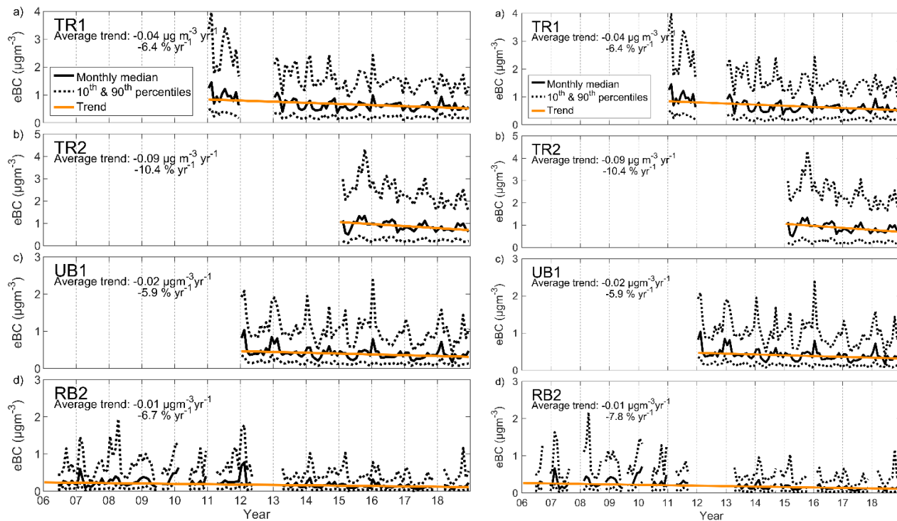
Figure 4: Time series and trends of eBC concentration at TR1, TR2, UB1, and RB2. The solid black line represents the monthly medians, the dashed lines represent the 10 th and 90 th monthly percentiles, and the orange line is the fitted long-term trend.
