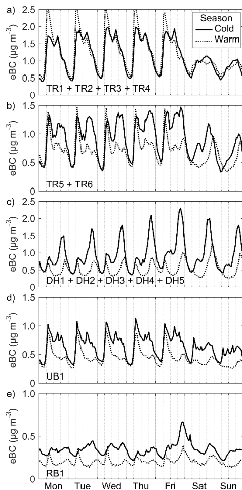
830 Figure 6: Diurnal variation of eBC for different station categories: a) traffic sites that were not influenced by wood burning (TR1–4), b) traffic sites that were influenced by wood burning (TR5–6), c) detached housing sites (DH1–5), d) urban background (UB1), and e) regional background (RB1). The diurnal variation is determined separately for the cold (from November to March) and warm (from May to September) periods.
