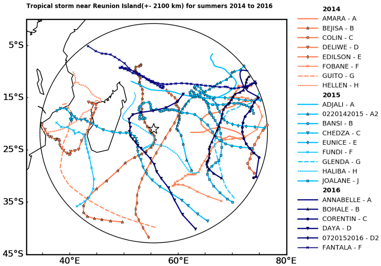
Figure 9: Map of Tropical Cyclone's best-tracks for a range ring of 2100 km around Réunion Island. The best-tracks of tropical Cyclones during austral summer 2014 (November 2013 to April 2014) are shown in orange with different symbols for each TC, best-tracks for austral summer 2015 (November 2014-April 2015) are in cyan and in blue for austral summer 2016 (November 2015-April 2016, in green). The yellow star indicates the location of Réunion Island.
