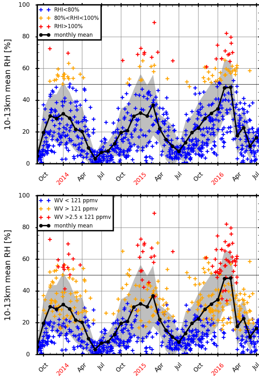
610 Figure 4: Top, daily evolution of mean upper tropospheric (10 to 13 km) RH for the period September 2013 to July 2016. The RH (with respect to water) values are color coded according to the values of RHi. In blue RH values for RHi < 80\% , in orange RH values for 80\% < RHi < 100\% , and in red RH values for RHi > 100\% . Bottom, daily evolution of mean upper tropospheric (10 to 13 km) 615 RH for the period September 2013 to July 2016. The RH (with respect to water) values are color coded according to the values of water vapor mixing ratios (WV). The mean 10-13km WV is 121 ppmv. In blue RH values for WV < 121 ppmv, in orange RH values for 121 \text{ ppmv} < WV < 2.5 \times 121 ppmv and in red RH values for WV > 2.5 \times 121 ppmv. On the two panels, the black thick line corresponds to the monthly mean RH in the upper-troposphere.
