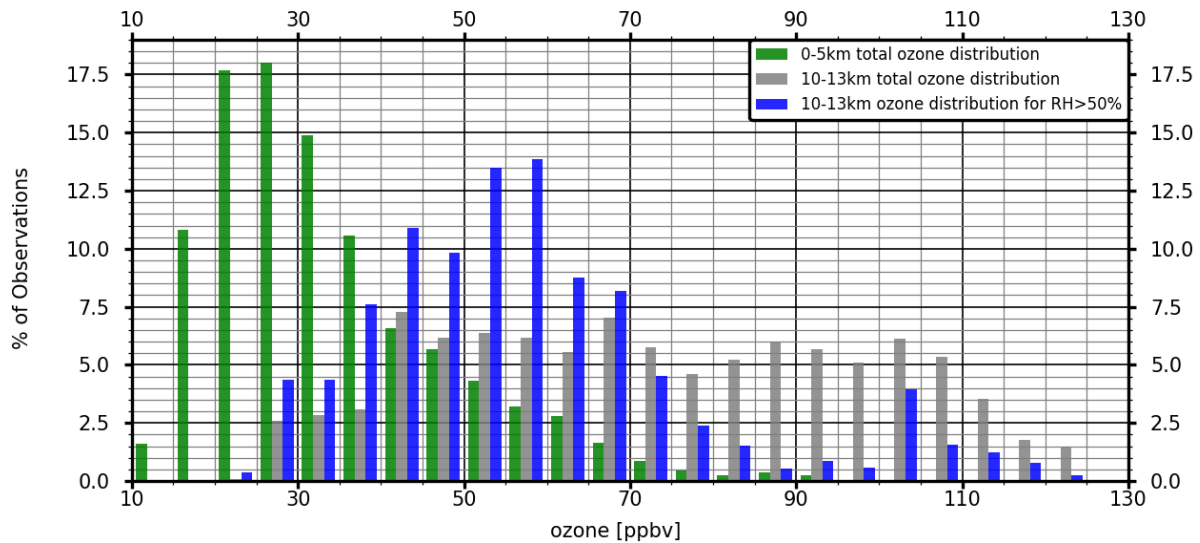
Figure 6: NDACC/SHADOZ ozone distribution in the lower troposphere (0-5 km, in green). The total distribution in the upper troposphere (10-13km, in grey) and for moist data (10-13km and RH>50%, in blue). The distributions are based on 55 ozone profiles for austral summers 2014, 2015 and 2016. The mean for each distribution is 73.8 ppbv, 57 ppbv, 33.5 ppbv for the 10-13 total ozone distribution, 10-13 km ozone distribution with RH>50% and 0-5km total ozone distribution respectively.
