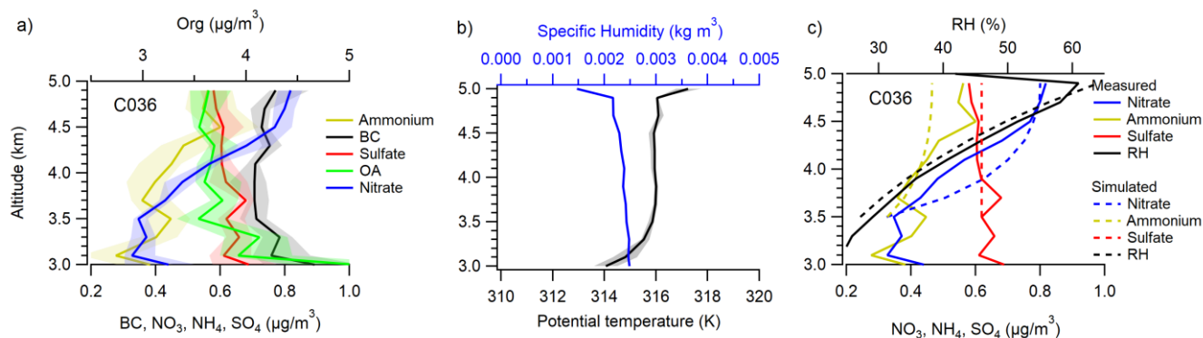
Figure 10: The vertical distribution (3000 – 5000 m) of a) different chemical composition concentrations and b) potential temperature and specific humidity in flight C036 (24 August). The lines and shades represent the 25%, median and 75% in every 200m bin. c) The simulated and measured chemical composition and RH at different altitudes with variable temperatures.
