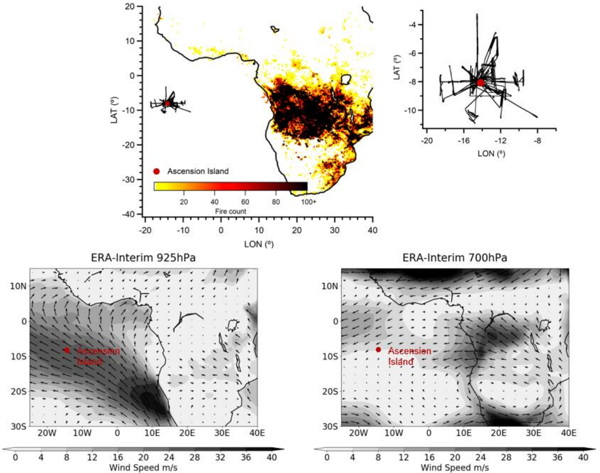
Figure 1: (Top panel) The integrated spatial distribution of MODIS-detected fire counts in August 2017, coupled with flight tracks (without transit flights) during CLARIFY-2017 aircraft campaign (16 th August-7 th September). (Bottom panel) Average wind speed and direction at 925hPa (left) and 700hPa (right) in ERA-Interim re-analysis for August 2017. The wind speed is shown in grey scale bars.
