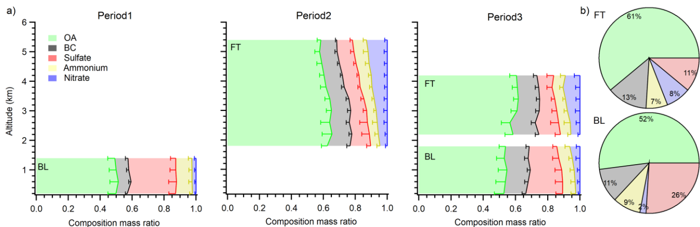
Figure 3: a) The average vertical distribution of PM1 chemical composition ratios in the BB-polluted FT and BL separately in each period. The width of color bars represents average mass ratio of different species in every 400 m bin. The error bars represent one standard deviation. b) Pie charts showing campaign-average chemical composition ratios in the BB-polluted FT and BL respectively.
