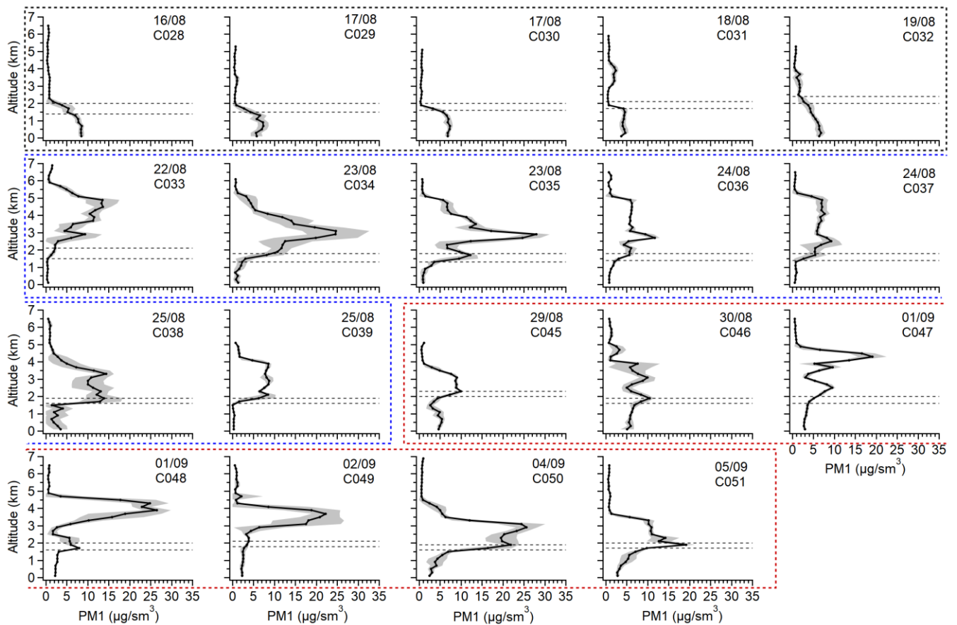
Figure 2: The average vertical distribution of submicron aerosol (PM1) in flights used in this study. PM1 is calculated from AMS non-refractory submicron species and SP2 BC. The grey shades represent standard deviation. The dashed lines represent the lower and upper level of the inversion layer. Period 1 is marked by black dashed square, which shows that BBA was concentrated in the BL. Period 2 is marked by blue, which shows that the FT was BB-polluted, and the BL was mostly clean. Period 3 is marked by red, which shows that the BB pollution was observed throughout the BL and FT.
