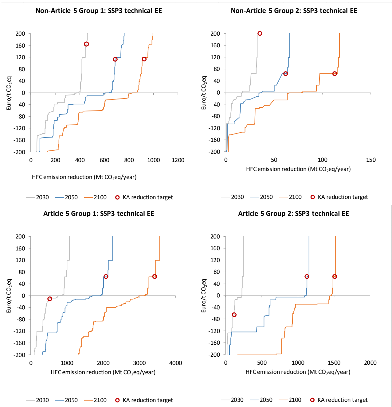
835 Figure 3: Marginal abatement cost curves (MACCs) starting from a pre-Kigali SSP3 baseline consistent with the IEA-WEO17 New Policies scenario and reducing HFC emissions by Kigali Amendment (KA) party groups under technical energy efficiency improvements and indicating the KA HFC reduction targets in 2030, 2050 and 2100.
