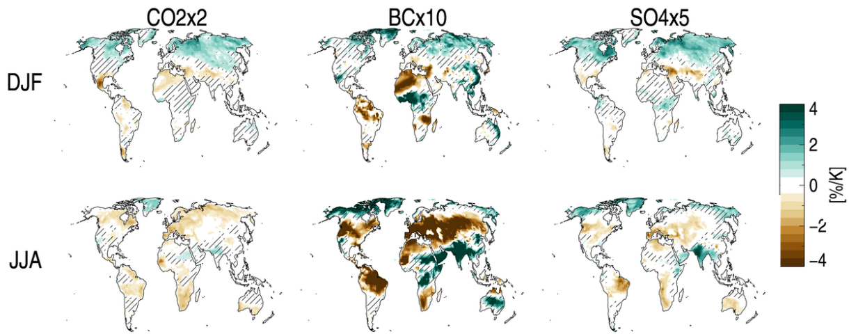
610 Figure 6: Multi-model median seasonal cloud cover change for the three drivers, normalized by the global annual mean temperature change. Hatching indicates that less than 75% of the models agree on the sign of the change.
