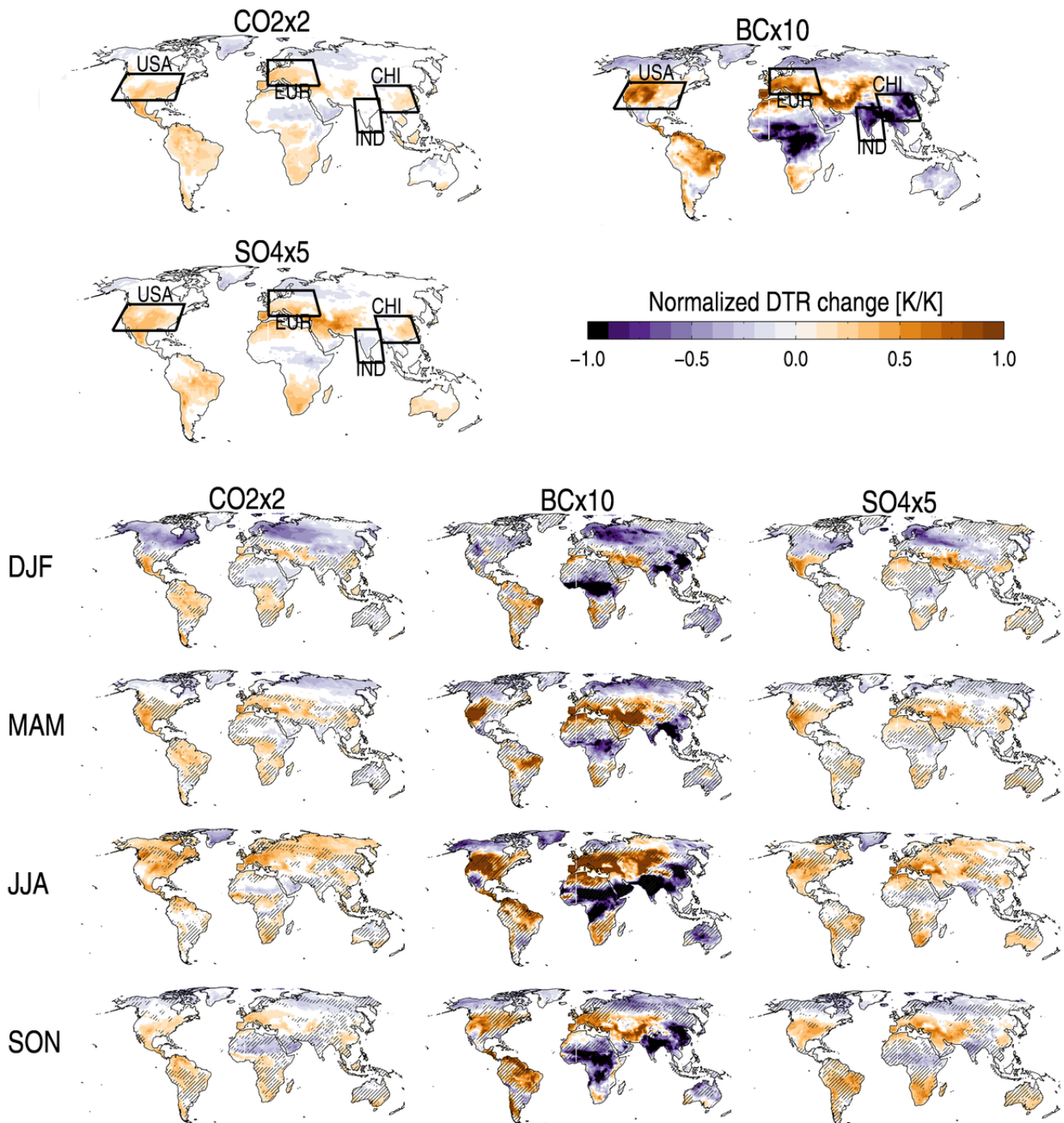
560 Figure 3: Multi-model median change in DTR, normalized by the global mean temperature change [K/K], for the three experiments. Large upper maps show annual mean changes, while smaller maps show seasonal changes. Hatching indicates areas where less than 75% of the models agree on the sign of the change. Annual maps include indications of the focus regions of this study. The region called “LND” throughout the manuscript is the average of all land regions on the globe.
