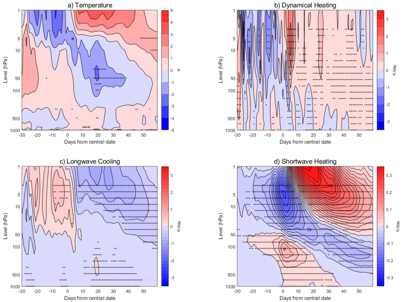
Figure S3. As in Figure 5, for March SSWs.
