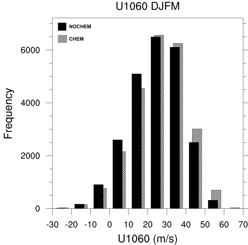
Figure 2. Histogram of daily values of zonal mean zonal wind at 10 hPa and 60°N in December-March for CHEM and NOCHEM. The mean and standard deviation of the CHEM and NOCHEM zonal mean zonal wind values are 26.5 26.1 m/s and 12.9 24.4 m/s. For NOCHEM, these values are 25.0 m/s and 12.3 m/s respectively. The shift to a stronger vortex in right tail of the CHEM compared to NOCHEM distribution is statistically significant at the 95% level based on longer, indicating more days of a Kolmogorov-Smirnov test; the difference in means is significant at the 95% level based on a two-sample t-test particularly strong polar vortex.
