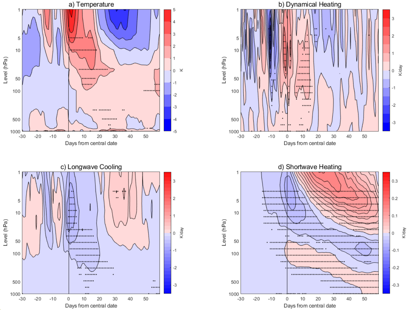
Figure 5. CHEM-NOCHEM differences in the temperature and heating anomalies over 60-90° N from -30 to +60 days around the SSW DJF central dates. Top-left(a): temperature-Temperature anomalies. Contours are every 1 K. Top-right(b): dynamical-Dynamical heating anomalies. Contours are every 0.5 K/day. Bottom-left(c): longwave-Longwave heating anomalies. Contours are every 0.25 K/day. Bottom-right(d): shortwave-Shortwave heating anomalies. Contours are every 0.02 K/day. Stippling shows significance at the 95% level under a two-tailed t-test.
