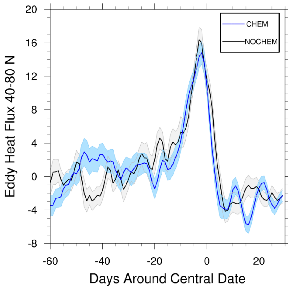
Figure S4. As in Figure 6, for March SSWs.
