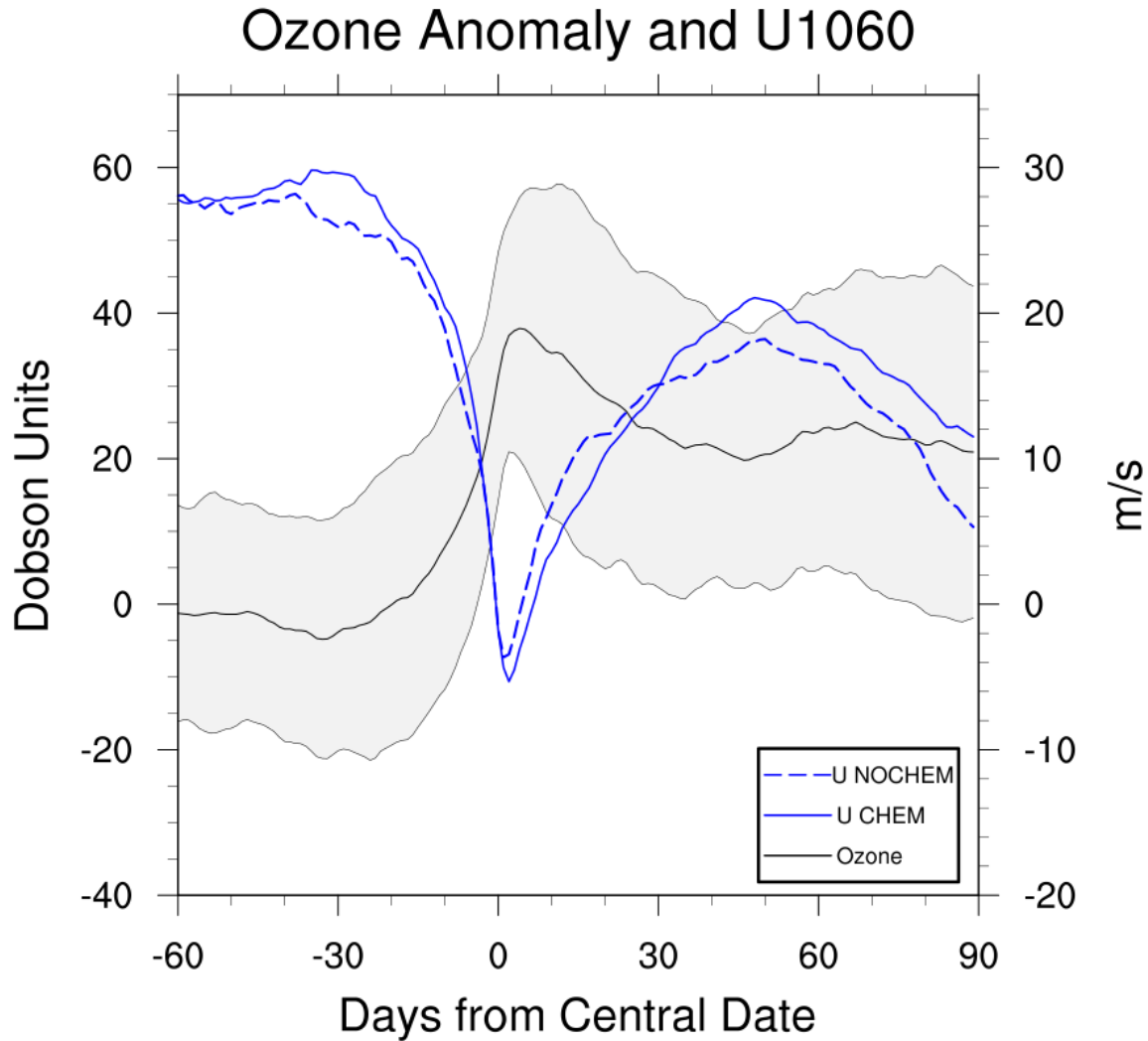
Figure 7. Composite of total column polar cap (over 60-90° N) ozone anomalies in Dobson units in the CHEM simulations and composite composites of zonal mean zonal wind at 60° N and 10 hPa in m/s from -60 to 90 days around the central date of DJF SSWs in CHEM simulations and NOCHEM. The black line shows the mean total ozone column; 1\sigma from the mean is shaded. The blue solid and dashed line shows the mean U1060 in CHEM and NOCHEM respectively.
