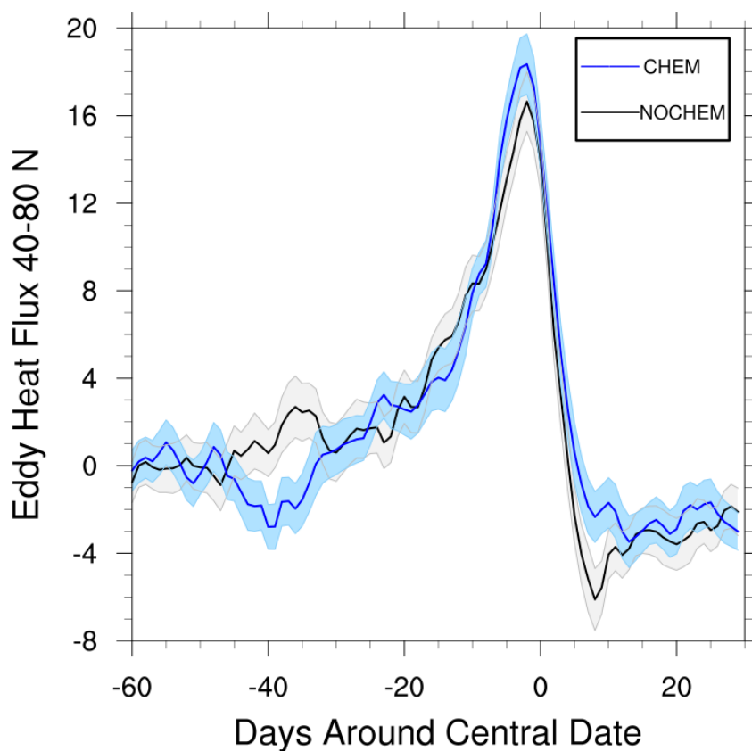
Figure 6. Eddy heat flux in shortwave heating anomalies \text{mK/s} over 40\text{--}80^\circ\text{ N} from -30\text{--}60 to +60\text{--}30 days around the SSW DJF central dates. The CHEM average is in December (top) blue, January (middle) with confidence intervals shown in pale blue. The NOCHEM average is in black, and February (bottom) with confidence intervals shown in gray.
