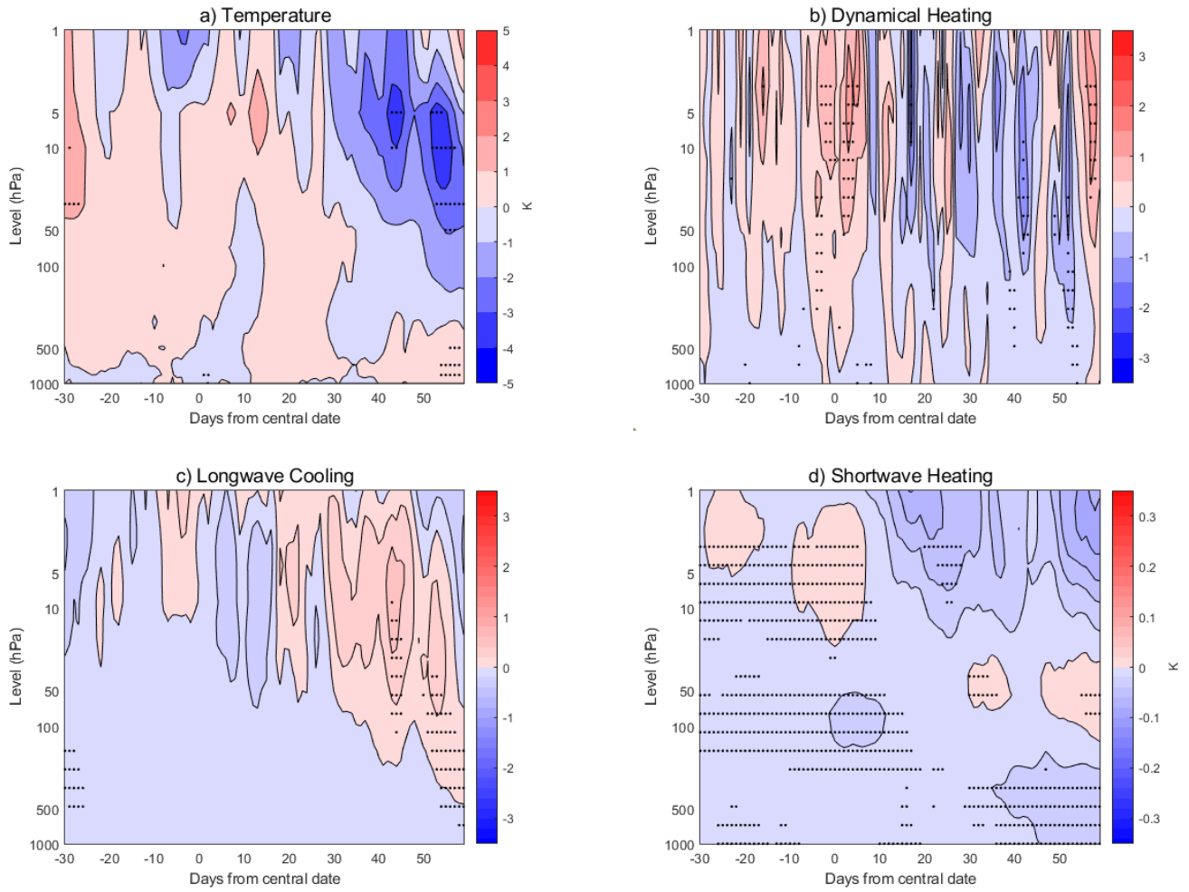
Figure S6. As in Figure 5, for DJF SPVs.
