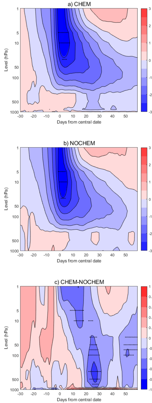
Figure 4. NAM anomaly composites around DJF SSW central dates in CHEM (topa), NOCHEM (middleb), CHEM-NOCHEM (bottomc). Stippling shows significance at the 95% level (with a Monte Carlo test for CHEM and NOCHEM and a two-tailed t-test for CHEM-NOCHEM). Contours are every 0.5 standard units for CHEM and NOCHEM and every 0.2 standard units for CHEM-NOCHEM.
