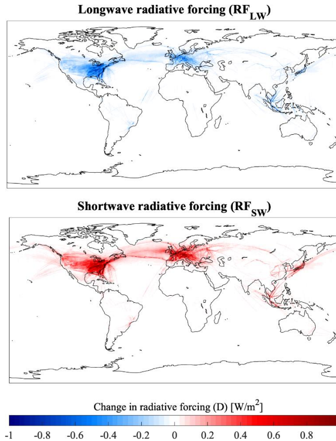
760 Figure 8. Change in annual-average RF [ W/m^2 ] due to the presence of clouds from global flights in 2015. Upper panel: Longwave RF (blue corresponds to negative, meaning that clouds reduce the warming effect of contrails). Lower panel: Shortwave RF (red corresponds to positive, meaning that clouds reduce cooling effect of contrails).
