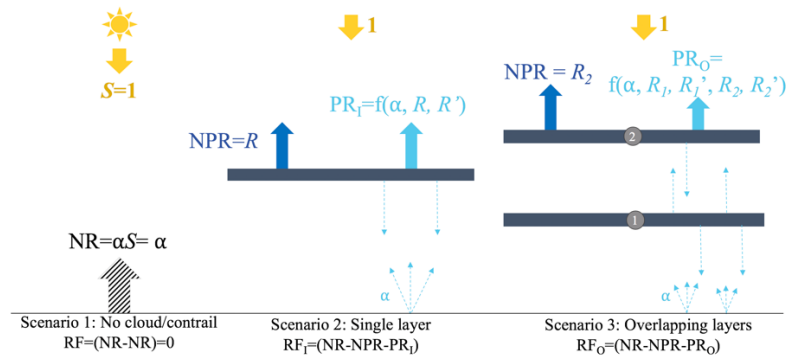
Figure D1. Components of response to a unit of incident light for 3 scenarios: no cloud/contrail, single layer, overlapping layers
