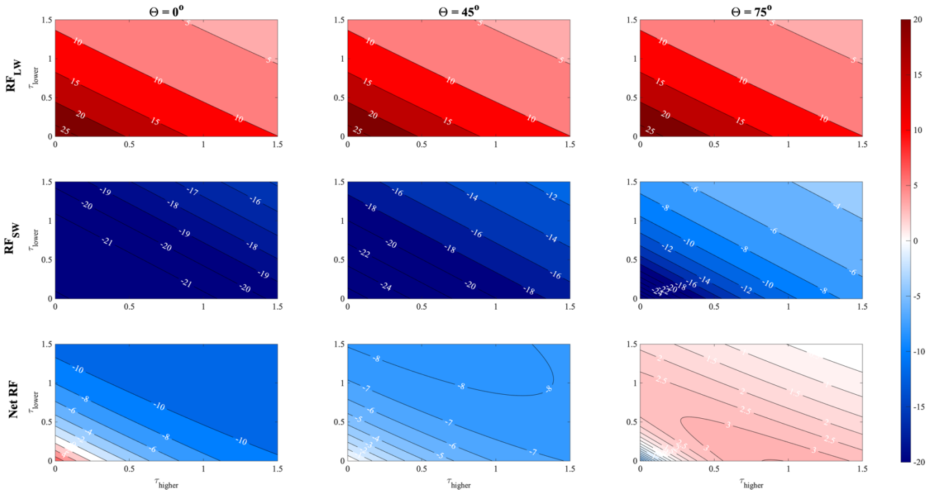
Figure 4. Radiative forcing [ \text{W}/\text{m}^2 ] due to a single contrail between two cirrus cloud layers. Radiative forcing is shown as a function of the solar zenith angle (increasing from left to right) and the optical depth of the lower (Y-axis) and upper (X-axis) natural cloud optical depths. From top to bottom: longwave; shortwave; and net radiative forcing. Contrail optical depth \tau = 0.3 . An additional version of this figure, including calculations using a solar zenith angle \theta = 30^\circ and using a smaller contrail optical depth, is provided as Figure S7 for comparison to other literature.
