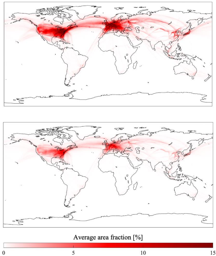
775 Figure 9. Estimated annual mean global contrail coverage for 2015. Upper panel: yearly average contrail coverage (in %), assuming no contrail-contrail overlap. Lower panel: yearly average coverage (in %), assuming “maximum overlap” such that all contrails in a single column are centered in each 0.25^{\circ} \times 0.3125^{\circ} grid cell (in %). Contrail data were generated using the CERM global contrail modeling tool (Caiazzo et al., 2017), which provides contrail quantities and properties discretized to the aforementioned global grid. More information on CERM can be found in Appendix A3. Maximum contrail overlap assumes that all contrails in a single vertical grid column overlap to the greatest possible extent by area. This estimate includes contrails which are diffuse and/or “sub-visible” (optical depth < 0.03 ).
