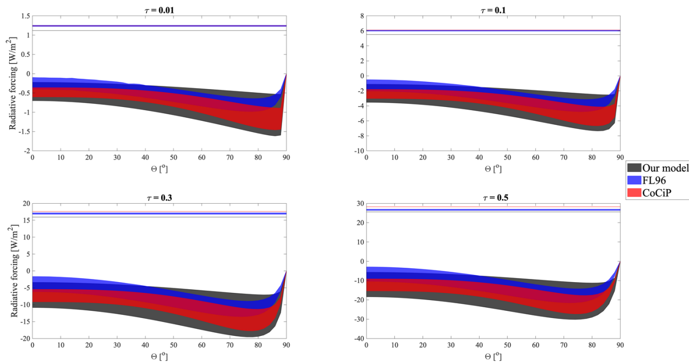
1460 Figure B1. Longwave (positive) and shortwave (negative) radiative forcing ranges (varying particle size) in \text{W}/\text{m}^2 with the three models tested here: our model (based on Corti and Peter), FL, and CoCiP. Variations with optical depth and solar zenith angle are shown.
