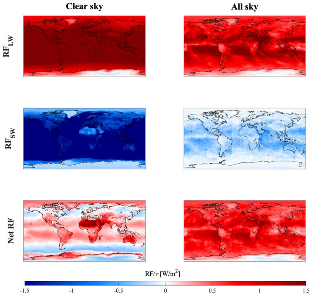
645 Figure 6. Hourly average radiative forcing per unit optical depth [ W/m^2 ] for a 1% contrail covering per 0.25^\circ \times 0.3125^\circ cell and g=0.77 (2015 atmospheric data) From top to bottom: Longwave, shortwave, and net RF. Clear sky sensitivities are shown on the left, and all sky calculations on the right. Small discontinuities in shortwave cooling for all-sky conditions (e.g. over the North Atlantic Ocean) are the result of data artifacts in the CERES satellite data, which is a composite of observations from multiple observation platforms.
