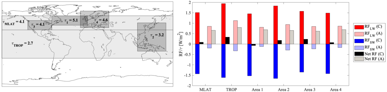
Figure 7. Contrail RF per unit of contrail optical depth for 6 different global areas: MLAT (northern midlatitudes), TROP (tropics), and subregions 1-4. Left panel: latitudinal and longitudinal limits and average natural cloud optical depth of each area. Right panel: average RF per unit of optical depth per area (A: all sky, C: clear sky).
