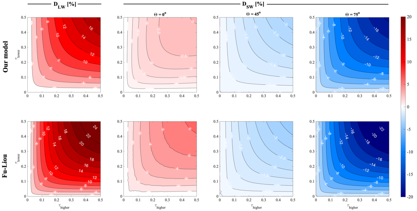
Figure 5. Error in estimated RF for two overlapping contrails when ignoring overlap, as a function of \tau and \theta , for both our model (upper row of panels) and FL (lower row of panels). The first column shows error in longwave RF, while the remaining columns show error in shortwave RF at different solar zenith angles. Positive (red) values indicate that the independent assumption results in an overestimate of warming effects (or underestimate of cooling effects). Negative (blue) values indicate that the independent assumption results in an overestimate of cooling effects (or underestimate of warming effects). An additional version of this figure, including calculations using solar zenith angles \theta = 15^\circ, 30^\circ and 60^\circ is provided as Figure S8 for comparison to other literature.
