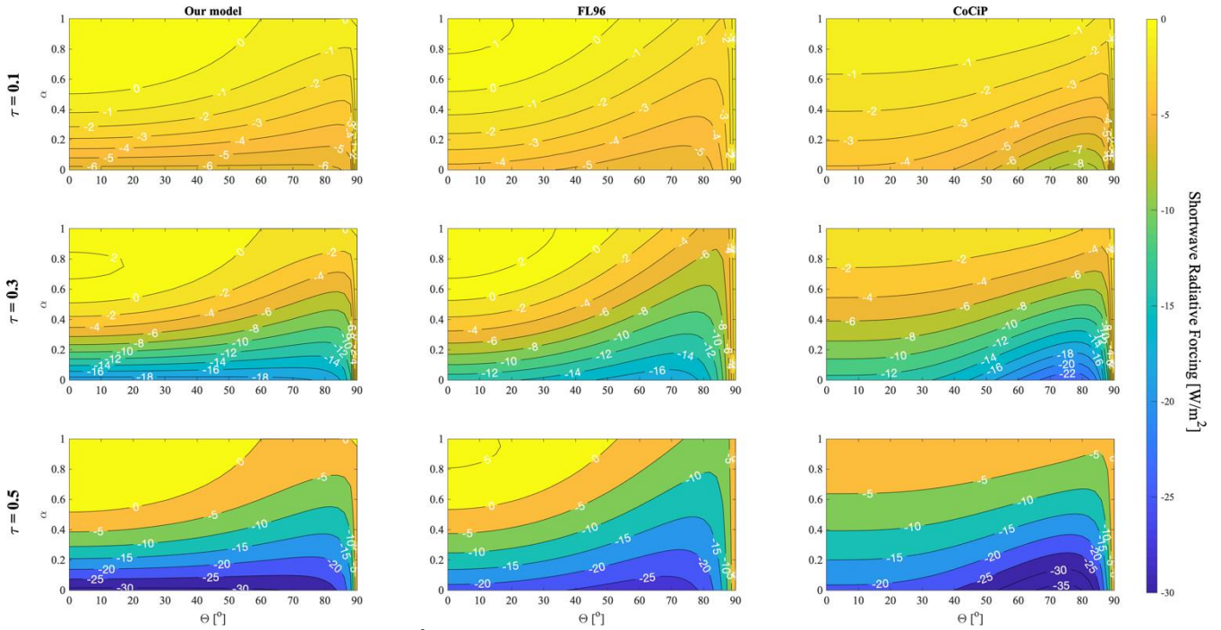
1515 Figure B2. Shortwave radiative forcing in \text{W/m}^2 of a single contrail as a function of surface albedo (Y-axis) and solar zenith angle (X-axis). Each column corresponds to a different model, and each row corresponds to a different contrail optical depth.
