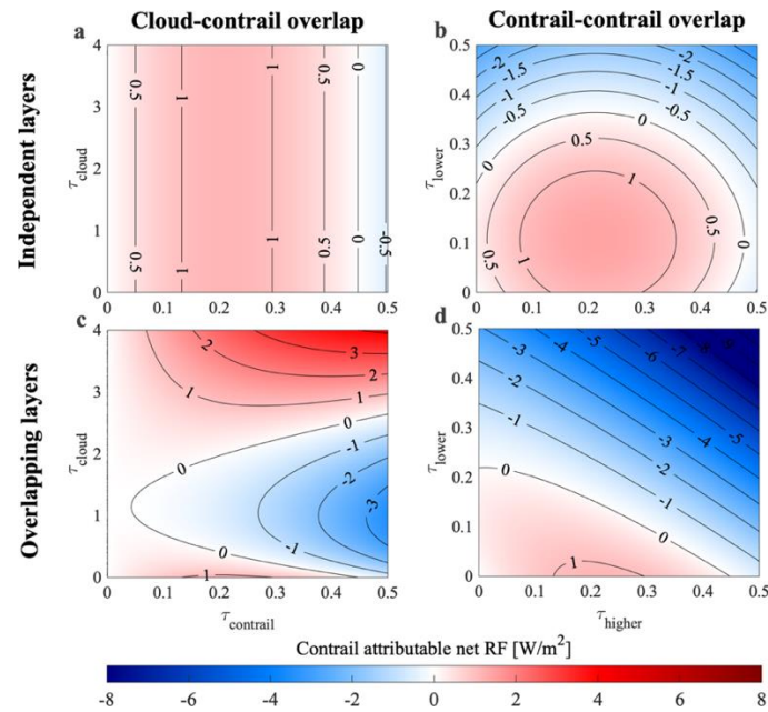
Figure 2. Effect of overlap between two layers on the contrail net RF as a function of optical depth \tau . Left: RF attributable to a single contrail 440 when overlapping with a natural cloud layer. Right: total RF in a system of two overlapping contrails. Top: contrail RF estimated when treating the layers as independent and summing individual contributions. Bottom: contrail RF estimated in a single calculation which 445 accounts for overlap. Negative RF is shown in blue and positive RF is shown in red. Contrail properties are: asymmetry parameter of 0.77, temperature of 220 K and 215 K respectively. Cloud properties are: asymmetry parameter of 0.85, temperature of 260 K. The solar zenith angle \theta = 45^\circ for all calculations. An additional version of this figure, calculated using a solar zenith angle \theta = 30^\circ and covering a greater range of optical depths, is provided as Figure S3 for comparison to other literature.
