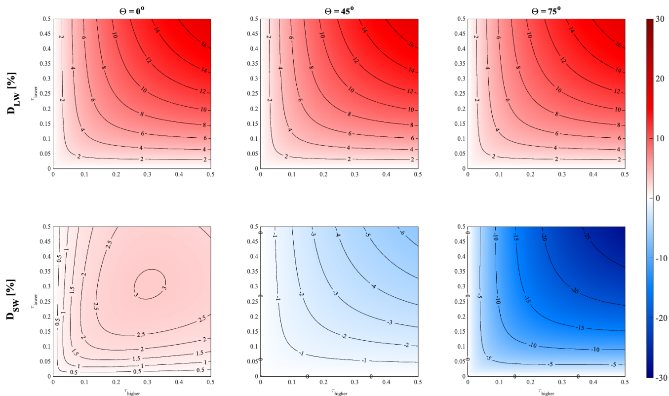
Figure 3. Error in estimated RF for two overlapping contrails when ignoring overlap, as a function of \tau and \theta . The solar zenith angle increases from the left-most to right-most panels. The upper panels show longwave RF error, while the lower panels show shortwave RF error. Positive (red) values indicate that the independent assumption results in an overestimate of warming effects (or underestimate of cooling effects). Negative (blue) values indicate that the independent assumption results in an overestimate of cooling effects (or underestimate of warming effects). An additional version of this figure, including calculations using a solar zenith angle \theta = 30^\circ and covering a larger range of contrail optical depths, is provided as Figure S6 for comparison to other literature.
