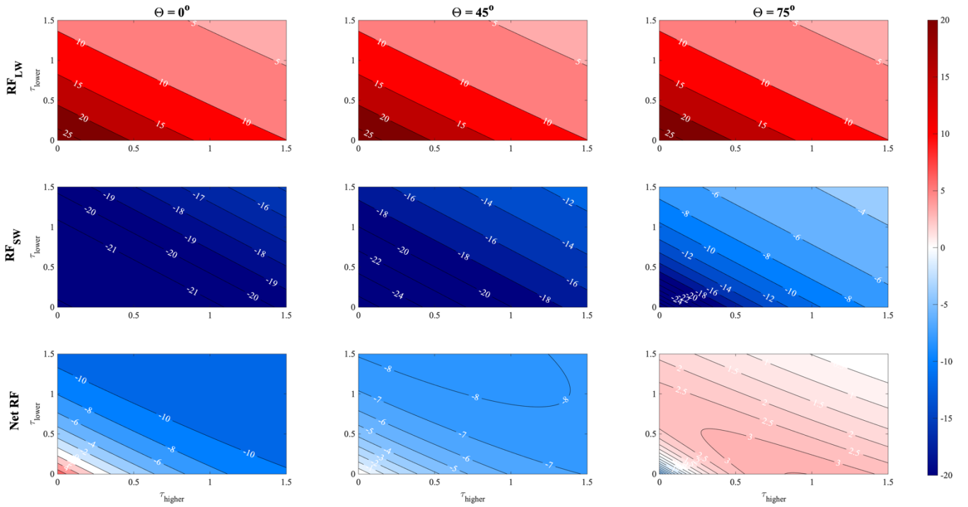
570 Figure 4. Radiative forcing [ \text{W/m}^2 ] due to a single contrail between two cirrus cloud layers. Radiative forcing is shown as a function of the solar zenith angle (increasing from left to right) and the optical depth of the lower (Y-axis) and upper (X-axis) natural cloud optical depths. From top to bottom: longwave; shortwave; and net radiative forcing. Contrail optical depth \tau = 0.3 . An additional version of this figure, including calculations using a solar zenith angle \theta = 30^\circ and using a smaller contrail optical depth, is provided as Figure S7 for comparison to other literature.
