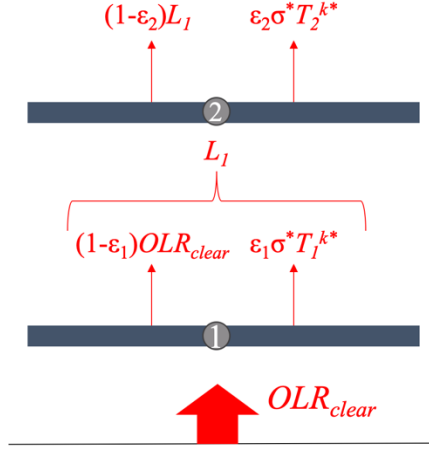
Figure 1. Schematic of longwave RF calculation in a two-layer overlap. Arrows represent emitted or transmitted longwave radiation. OLR_{clear} is the longwave emission from the Earth's surface, while L_i is the longwave emission from layer i . \epsilon_i and T_i are emissivity and temperature of each of the layers.
