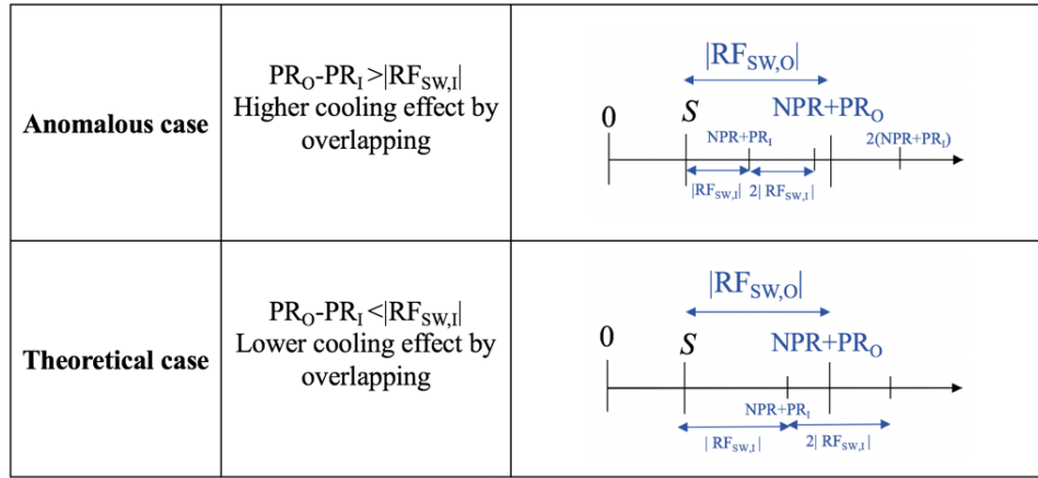
Figure D2. Comparison scheme of reflection components in an overlap (Upper case: increase in cooling; lower case: decrease in cooling)
