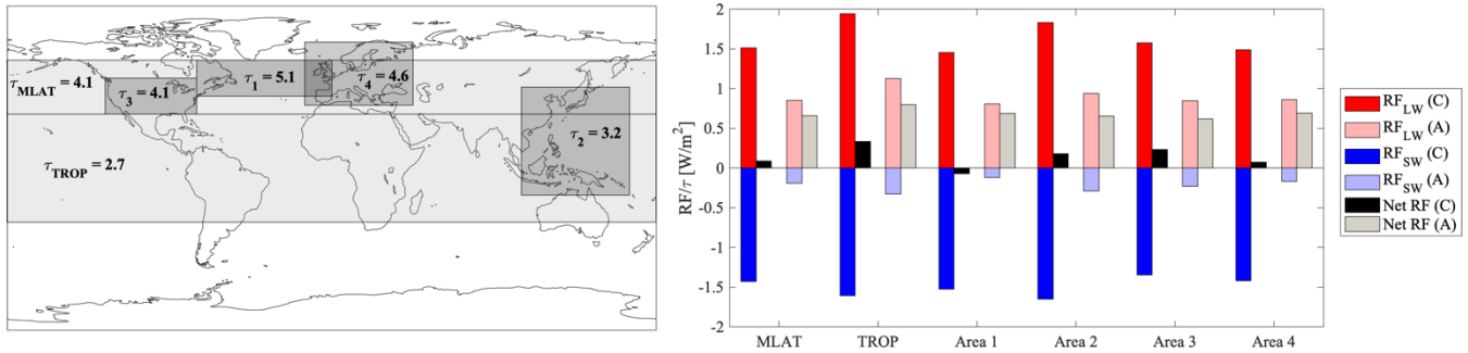
Figure 7. Contrail RF per unit of contrail optical depth for 6 different global areas: MLAT (northern midlatitudes), TROP (tropics), and subregions 1-4. Left panel: latitudinal and longitudinal limits and average natural cloud optical depth of each area. Right panel: average RF per unit of optical depth per area (A: all sky, C: clear sky).
