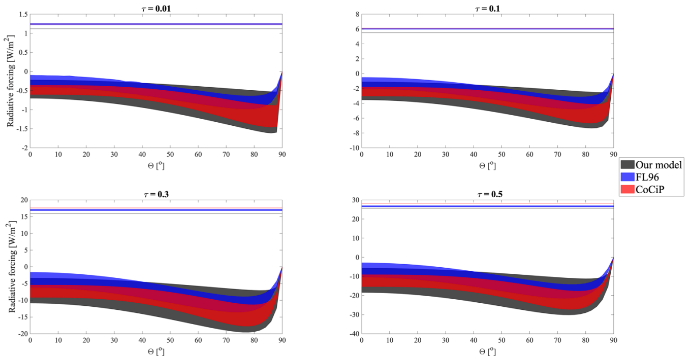
Figure B1. Longwave (positive) and shortwave (negative) radiative forcing ranges (varying particle size) in \text{W}/\text{m}^2 with the three models tested here: our model (based on Corti and Peter), FL, and CoCiP. Variations with optical depth and solar zenith angle are shown.
