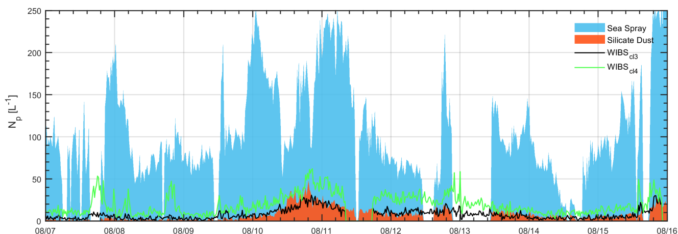
Figure 7. Time series of sea spray aerosol and silicate dust particle numbers concentrations determined by LAAP-ToF and WIBS-4A clusters C13 & C14. 20 Minute averages have been used here.
