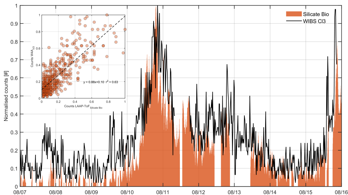
Figure 9. Time series of WIBS Cl3 and silicate dust filtered for Bio markers using 20 minute averaged number counts normalised by the maximum observed concentration for each instrument.
