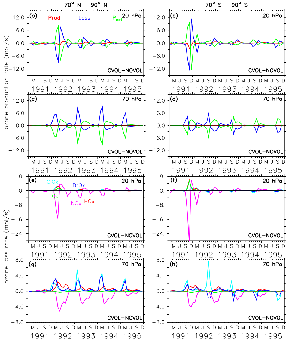
Figure 12. Chemical effect (CVOL-NOVOL) of ozone production (Prod) and loss (Loss) rates (a)-(d) in polar regions and corresponding net ozone production ( P_{\text{net}} = \text{Prod} - \text{Loss} ). (a) (20 hPa) and (c) (70 hPa) show zonally averaged and latitudinally ( 70^\circ \text{ N} and 90^\circ \text{ N} ) summed rates in mol/s. (b) and (d): similar as for (a) and (c), but for 70^\circ \text{ S} - 90^\circ \text{ S} . The shown levels are located in the maximum of the volcanic ozone perturbation. Chemical effect (CVOL-NOVOL) of the zonally averaged and latitudinally summed ozone loss rates (mol/s) for each catalytic ozone loss cycle (e)-(h) for the polar region at 20 hPa (e) and 70 hPa (g). (f) and (h) are similar to (e) and (g), but for 70^\circ \text{ S} - 90^\circ \text{ S} , respectively.
