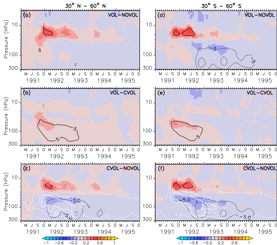
Figure 8. Colours show the zonally averaged differences of ozone mixing ratios (ppmv) between the simulations VOL - NOVOL (a) and (d), VOL-CVOL (b) and (e) and CVOL-NOVOL (c) and (f). Contours indicate the corresponding relative changes (%). Shown are averages over the mid latitudes 30° N - 60° N (left) and 30° S - 60° S (right). Contour intervals are 5 %. White contours in (c) show the liquid aerosol surface area density ( 10^{-8} \text{ cm}^2 \text{ cm}^{-3} ) in VOL and CVOL with intervals of 1.5 and 10.
