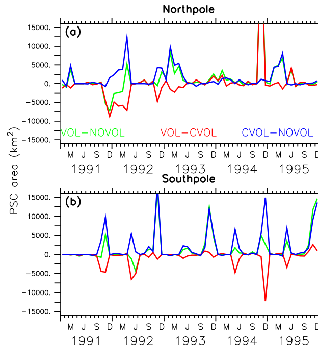
Figure 15. Differences of polar stratospheric cloud (PSC) covered area ( \text{km}^2 ) at the Northpole North Pole (a) and Southpole South Pole (b) for the combined effect (green), the heating effect (red) and the chemical effect (blue).
