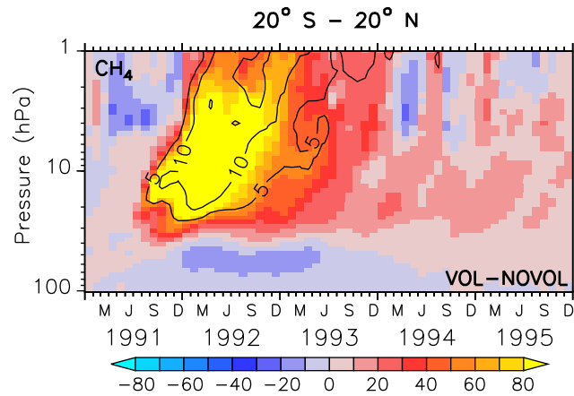
Figure 17. Colours show the zonally averaged differences of the methane mixing ratio (ppbv) for the combined effect (VOL-NOVOL). The black contours show the relative change (%) of methane in comparison to NOVOL. Shown are tropical averages (20° S - 20° N). Contour intervals are 5 %.
