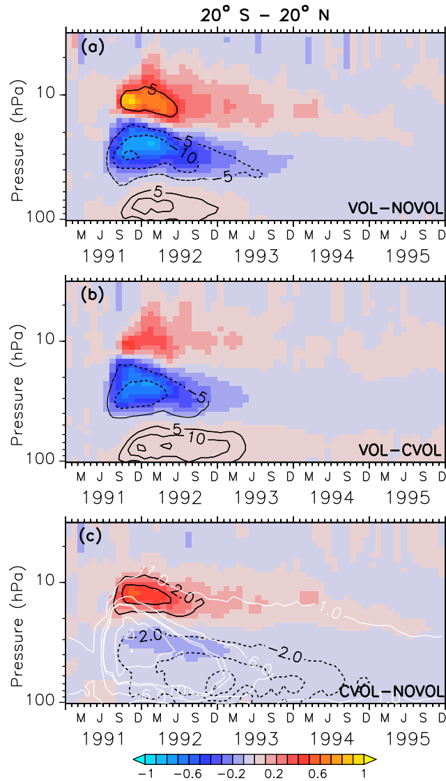
Figure 7. Colours show the zonally averaged differences of ozone mixing ratios (ppmv) between two simulation results, where (a) shows the combined effect (VOL-NOVOL), (b) the heating effect (VOL-CVOL), and (c) the chemical effect (CVOL-NOVOL). Black contours indicate the corresponding relative changes (%). Shown are averages in the tropics between 20° S and 20° N. Contour intervals are 5 % in the upper and central panel, and 2 % in the bottom panel. White contours in (c) show the liquid aerosol surface area density ( 10^{-8} \text{ cm}^2 \text{ cm}^{-3} ) in VOL and CVOL with intervals of 1, 5 and 10.
