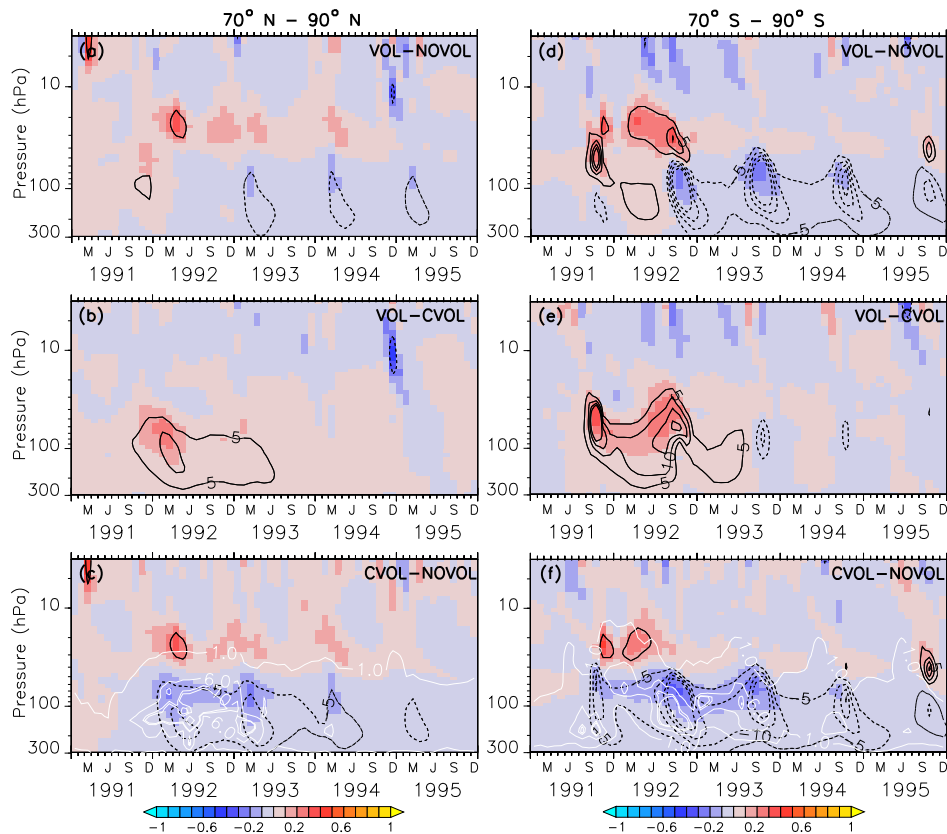
Figure 9. Colours show the zonally averaged differences of ozone mixing ratios (ppmv) between the simulations VOL - NOVOL (a) and (d), VOL-CVOL (b) and (e) and CVOL-NOVOL (c) and (f). Contours indicate the corresponding relative changes (%). Shown are averages over the mid latitudes 70° N - 90° N (left) and 70° S - 90° S (right). Contour intervals are 5 %. White contours in (c) show the liquid aerosol surface area density ( 10^{-8} \text{ cm}^2 \text{ cm}^{-3} ) in VOL and CVOL with intervals of 1, 5 and 10.
