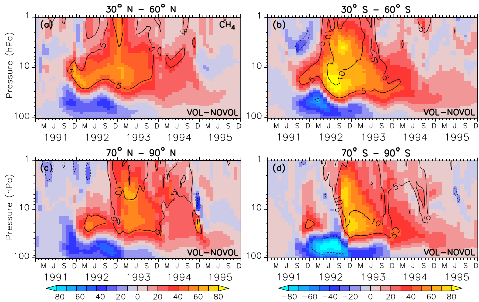
Figure 18. Colours show the zonally averaged differences of methane (ppbv) of the combined effect (VOL-NOVOL). The black contours show the relative change (%) of methane in VOL comparison to NOVOL, respectively. Shown are extratropical averages ((a) and (b)) (a) and (b): 30° N - 60° N and 30° S - 60° S; (c) and (d) (c) and (d): 70° N - 90° N and 70° S - 90° S). Contour intervals are 5 %.
