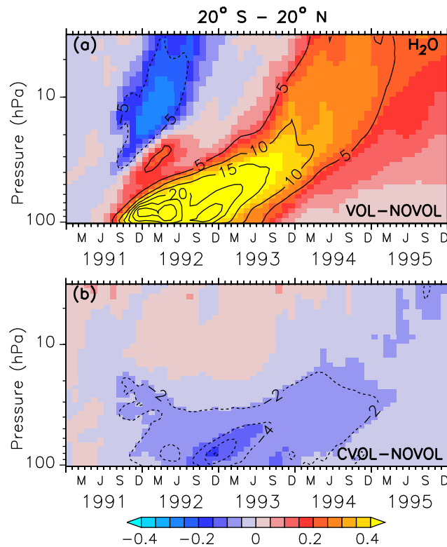
Figure 16. Colours show the zonally averaged differences of stratospheric water vapour (ppmv) between the simulations, where (a) shows the combined effect (VOL-NOVOL) and (b) the chemical effect (CVOL-NOVOL). The black contours show the relative change (%) of water vapour in comparison to NOVOL and CVOL, respectively. Shown are tropical averages ( 20^{\circ} S - 20^{\circ} N). Contour intervals are 5 % (a) and 2 % (b).
