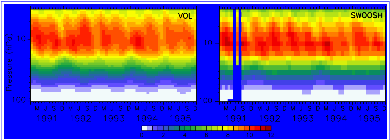
Figure 3. Colours show the absolute zonally and monthly averaged ozone mixing ratios (ppmv) at 10^{\circ} N of the volcanic simulation VOL (left) and the SWOOSH satellite data set (right) for the period from 1991-1995 (Davis et al., 2016).
