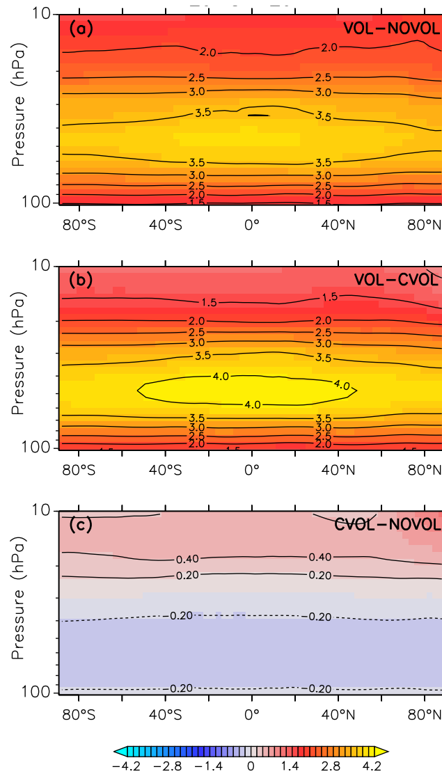
Figure 5. Colours show Monthly mean of the zonally averaged stratospheric temperature differences difference (K) between the model simulations of the stratosphere in (CVOL and NOVOL) for December 1991 as a monthly mean latitudinal cross section. 1991. (a) shows the combined effect, (b) the heating effect and (c) the chemical effect. Black contours indicate the isothermal curves (K). Contour intervals are 0.5 K in (a) and (b), and 0.2 K in (c).
