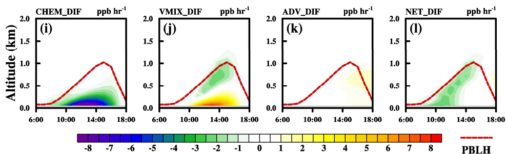
530 Figure 6: Averaged vertical distributions of processes contributions in function with time from 06:00 to 18:00 LT. (a)-(d) for CASE1; (e)-(h) for CASE2; (i)-(l) for the changes of each process contribution due to aerosols (Exp2-Exp1). Red dash lines denote PBLH.
