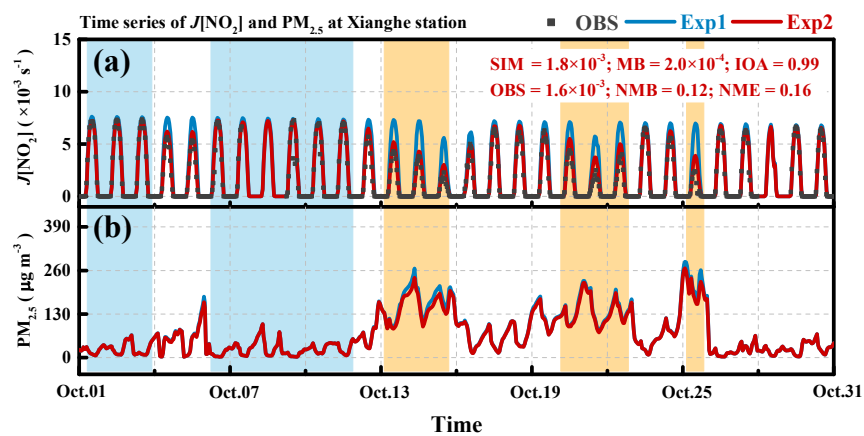
Figure 2: Time series of simulated J[\text{NO}_2] (a) and \text{PM}_{2.5} (b) at Xianghe station.
