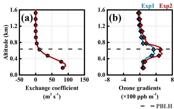
535 Figure 7: Averaged vertical profiles of (a) turbulence exchange coefficients and (b) vertical gradients of ozone from Exp1 and Exp2 at 12:00 AM. Dark gray dash line denotes PBLH at this time.
