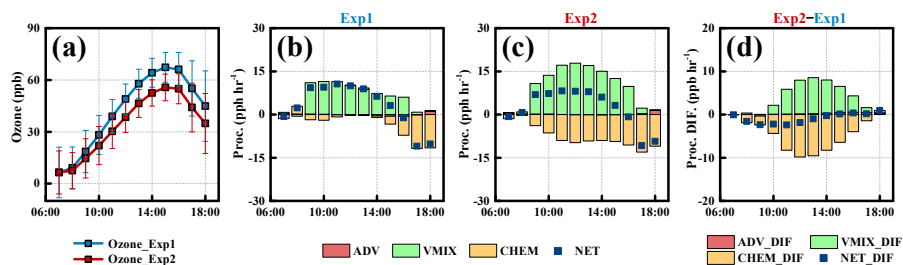
525 Figure 5: Averaged ozone concentrations at surface (a), hourly processes contributions and net contribution of ozone in Exp1 (b) and Exp2 (c), the changes of hourly processes contributions and net contribution induced by aerosol (Exp2-Exp1) at daytime. CHEM = chemistry, VMIX = vertical mixing, ADV = advection, NET = CHEM + VMIX + ADV. Changes of each process contribution and NET contribution are denoted by CHEM_DIF, VMIX_DIF, ADV_DIF and NET_DIF, respectively.
