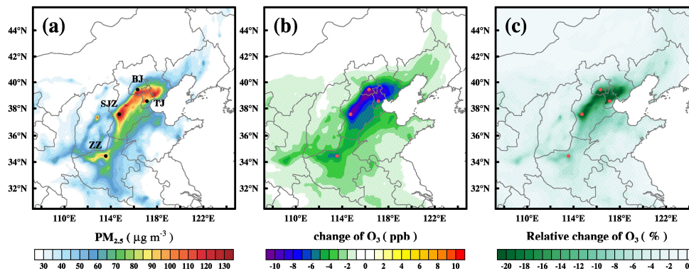
520 Figure 4: Mean distributions of \text{PM}_{2.5} (a), change of \text{O}_3 (b) and relative change of \text{O}_3 (c) at surface over CEC during high \text{PM}_{2.5} episodes. Dots denote the four typical cities in CEC, BJ=Beijing; TJ=Tianjin; SJZ=Shijiazhuang; ZZ=Zhengzhou
