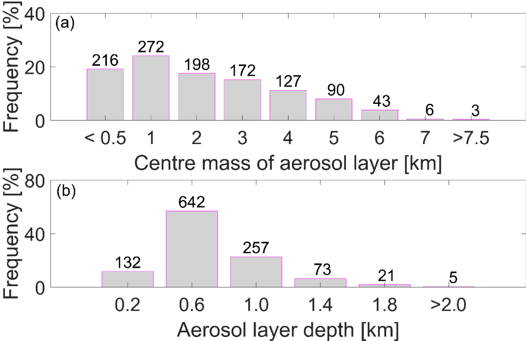
585 Figure 3. Geometrical characteristics of the aerosol layers during the campaign period. (a) Frequency of the altitude of the centre of mass of the aerosol layers. The width of each bin 1 km apart from the first and last bins. (b) Frequency of the geometrical depth of the aerosol layers. The width of each bin is 0.4 km apart from the last bin. The numbers on top of the bars indicates the amount of cases included in the bin.
