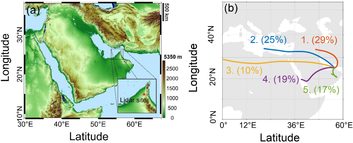
Figure 1. (a) Digital Elevation Map (DEM) from the NASA Shuttle Radar Topographic Mission ( SRTM ) for the greater area under study. The colorbar values correspond to the altitude above sea level. The site location is shown at the bottom-right of this figure with a red star. (b) Cluster analysis of sources of the detected night-time aerosol layer in the region computed with HySPLIT over the course of the campaign period. Colored lines indicate the trajectory path and the numbers show the percentage share of each trajectory path.
