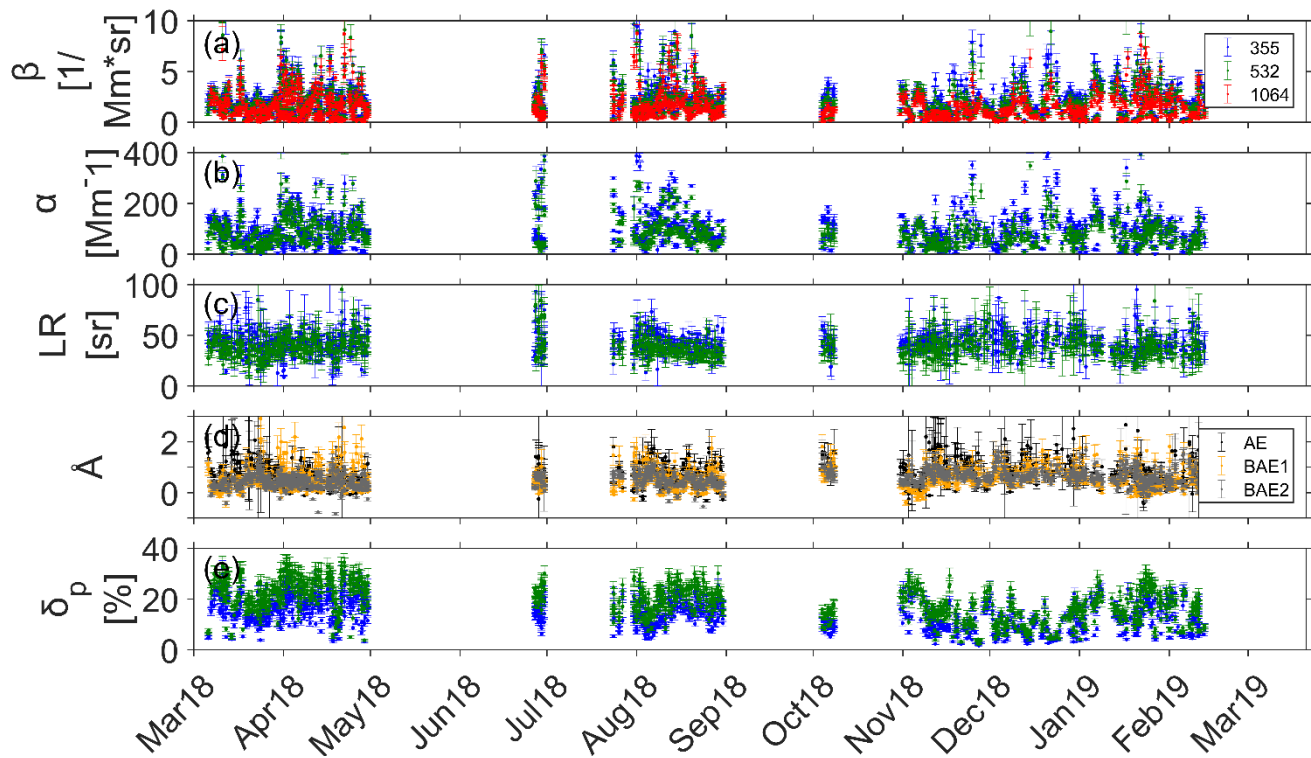
640 Figure 5. Timeseries of intensive and extensive aerosol properties at different wavelengths (355 nm in blue, 532 nm is green and 1064 nm in red). (a) Backscatter coefficient. (b) Extinction coefficient. (c) Lidar ratio. (d) Ångström exponents (Å) where the extinction-related Ångström exponent (AE) is marked with black dots, the backscatter -related Ångström exponent at 355/532 (BAE1) with orange and the backscatter-related Ångström exponent at 532/1064 (BAE2) with grey. (e) Linear particle depolarization ratio ( \delta_p ). The values show the mean optical property of the aerosol 645 layer along with one standard deviation indicated with the error bars.
