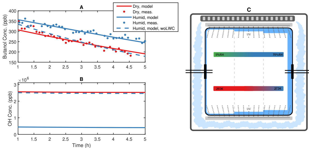
Figure 1. Illustration of the water film effect in the AURA chamber. Panel A depicts the PTR-MS butanol decay and B the OH concentration at varying RH with and without the influence of a liquid water film. The water content changed in accordance with varying temperature and RH, panel C. Outside cooling of the chamber may affect the water adsorption on the Teflon surface.
