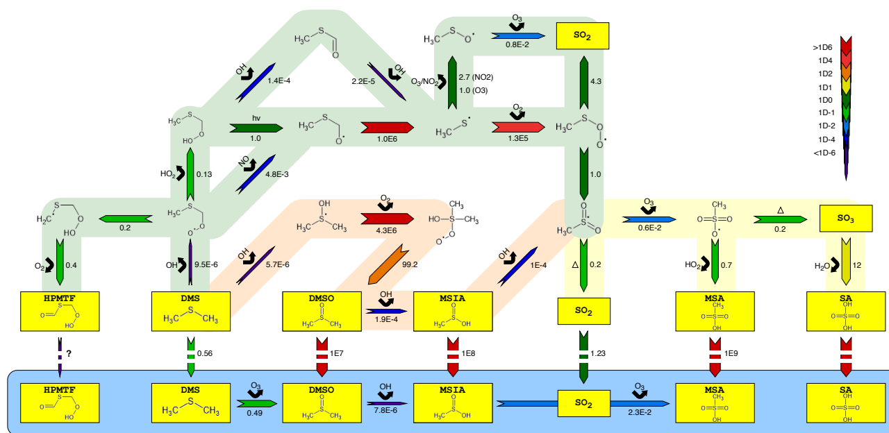
Figure 2. Simplified mechanism of the OH-initiated oxidation of DMS. Reaction rates are reported in s^{-1} for gas-phase and aqueous-phase chemistry, and M \text{ atm}^{-1} for phase-transfers (marked with broken arrows). All have been estimated at 293K, 5% RH and relevant OH, O_3 , HO_2 , NO and NO_2 concentrations in the AURA smog chamber. The blue area denotes the aqueous-phase oxidation of important water soluble intermediates and products (marked in yellow). Red and green shaded areas represent the OH addition and H abstraction pathways, respectively, while the yellow area illustrates the remaining mechanism after the two previous pathways intercept. The number beneath each arrow denotes the rate of said reaction, and the chemical species above its reactant.
