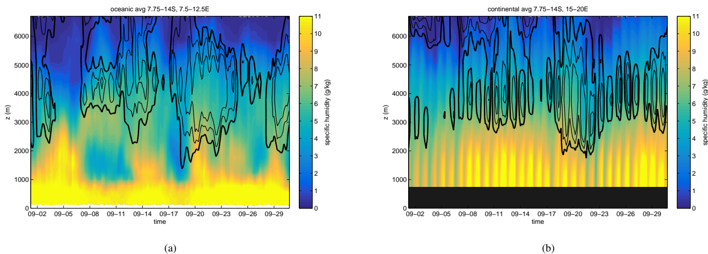
Figure 10. Oceanic (a) and continental (b) specific humidity (shaded) overlaid with zonal wind speed (black contours) from the ERA5 reanalysis. The thick black lines indicate the threshold of the AEJ-S (6 m/s) with thin black lines showing 8 and 10 m/s easterly velocities.
