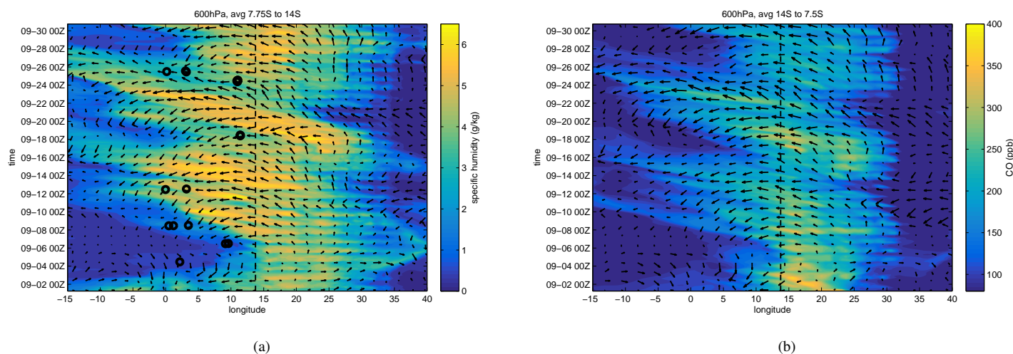
Figure 9. Hovmöller plot showing the development and transport of airmasses from continental Africa over the SEA, with colors showing a. water vapor from ERA-5, and b. carbon monoxide from MERRA-2, at 600hPa ( \sim 4.4 km), based on 3-hourly timesteps. The location of the African shoreline in this region is indicated by the black dashed line, and data are averaged between 7.75^\circ and 14^\circ S (note the domain is slightly larger for MERRA-2 due to the model resolution). Black circles show the locations and times of ORACLES aircraft profiles within this region. In the east (right-hand) of each plot, the diurnal convection cycle is evident, showing increased water vapor (CO) at this altitude during the daytime; in the west (left-hand), episodes of water vapor (CO) are seen as these continental airmasses are advected by the AEJ-S. Wind vectors do not scale between the two panels, although the patterns are seen to be largely similar between the two reanalyses.
