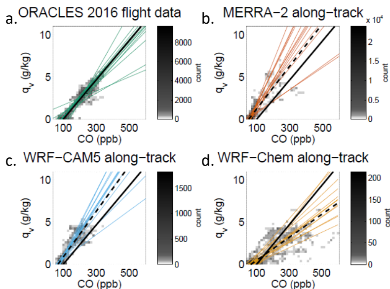
Figure 7. CO vs q from a. aircraft observations ( R^2 = 0.78 ), b. MERRA-2 reanalysis ( R^2 = 0.56 ), c. WRF-CAM5 ( R^2 = 0.71 ), and d. WRF-Chem ( R^2 = 0.49 ) for all flights, for altitudes z > 2 km. Individual colored lines show the total least-squares fits for individual flights, and the black lines show the averages of all observed flights (solid) compared to each model (dashed).
