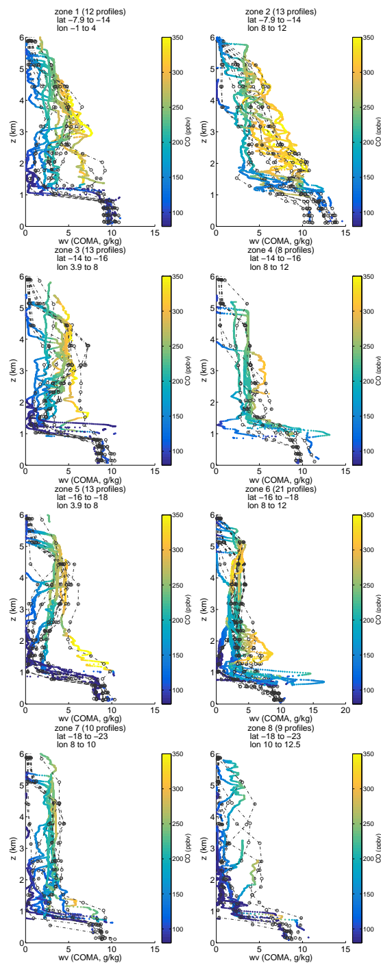
Figure 8. Profiles of specific water vapor measured by COMA in ORACLES-2016 (solid lines), subdivided by spatial location. Colors indicate the CO concentration from COMA. Dot-dashed lines show spatiotemporally co-located ERA5 reanalysis profiles for each aircraft profile, which captures the variability in vertical structure reasonably well.
