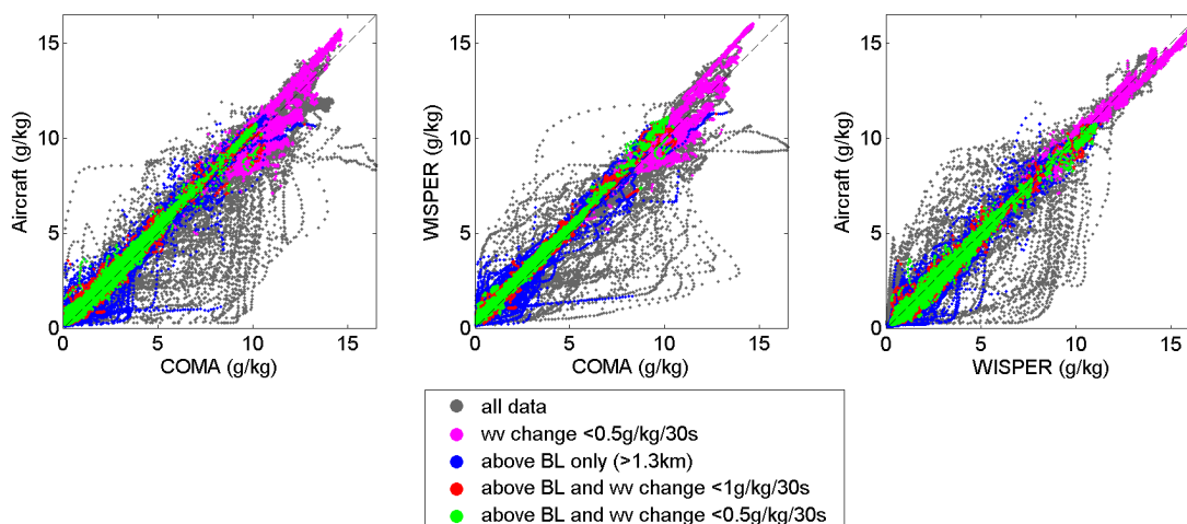
Figure 2. Comparison of water vapor specific humidity q from the three instruments for ORACLES-2016, for all flight data and for subsets based on altitude or change of water vapor with altitude. This subsetting highlights that the majority of the disagreement between instruments (grey dots) is either within the planetary boundary layer and/or during aircraft ascents/descents through rapidly changing conditions.
