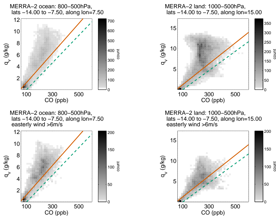
Figure 13. MERRA-2 CO and water vapor over land and over ocean, for (top) all observations along 15^{\circ}\text{E} and 7.5^{\circ}\text{E} , and (bottom) only observations for which easterly wind speed was >6\text{m/s} . For orientation with previous results, the green dashed line is the fit through all ORACLES-2016 free troposphere flight data and the solid red line shows the MERRA-2 fit coincident with the aircraft observations (both as in Figure 7). A vertically-resolved version of this plot is shown in Figure S5. The results are largely similar for WRF-CAM5 and WRF-Chem (Figure S6).
