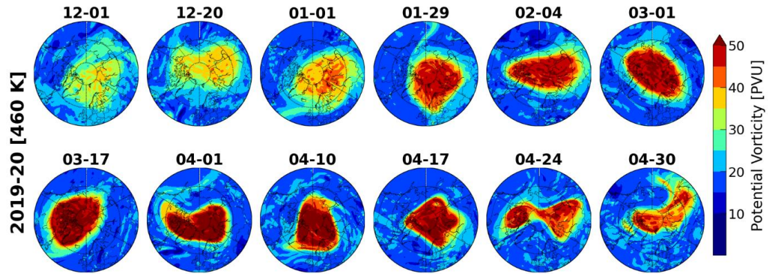
Figure 2: Polar vortex evolution in the Arctic winter/spring 2020. The evolution of polar vortex in the Arctic winter 2020. The vortex situation in the lower stratospheric altitude of about 460 K (~17 km) is illustrated. The vortex edge is calculated with respect to the Nash et al. (1996) criterion at each altitude.
