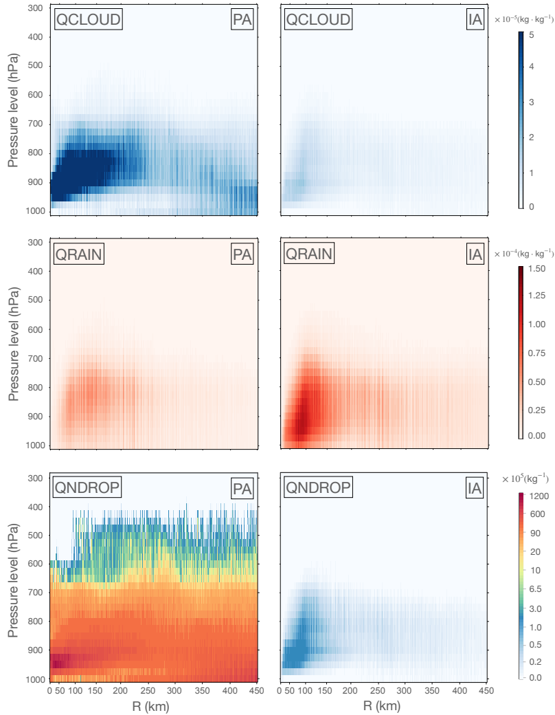
Figure 7. From top to bottom, cloud water mixing ratio (QCLOUD, kg\ kg^{-1} ), rain water mixing ratio (QRAIN, kg\ kg^{-1} ) and droplet number mixing ratio (QNDROP, kg^{-1} ). Time- and azimuthally-averaged height-radius cross sections are presented, for PA (left column) and IA (right column) simulations of Rolf starting with 36 hours of run-up time (i.e., on 2011 November 05 00:00 UTC), both without spectral nudging. Distance from the medicane center is represented in the horizontal axis and atmospheric pressure levels in the vertical axis. The three scales must be multiplied by the factor preceding the units in the legends titles.
