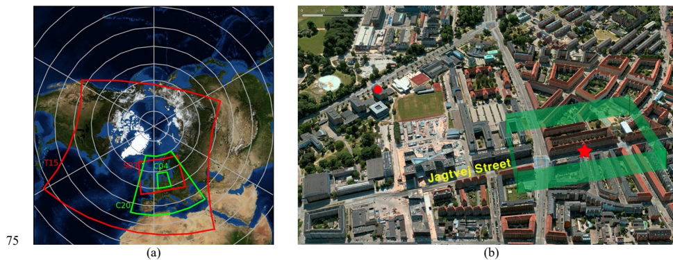
80 Figure 1: (a) operational and research modelling domains for European regional-scale (HIRLAM-T15+CAMx-C20) and sub-regional/urban Denmark scale (HIRLAM-S03+CAMx-C04) forecasts; (b) Nørrebro district of Copenhagen urban area with 2 air-quality monitoring stations, where red circle indicates a roof level air-quality observation at H.C. Ørsted Institute and red star indicates Jagtvej Street level observation; the green trapezoid shows M2UE modelling domain (extracted from © Apple Maps 2020).
