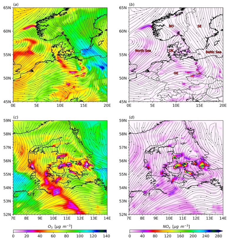
295 Figure 3: Simulation output on 5 Sep 2011, 10 UTC: HIRLAM-T15+CAMx-C20 results for concentrations in [ \mu g m^{-3} ] of (a) O_3 and (b) NO_x within the European regional-scale domain and HIRLAM-S03+CAMx-C04 results for concentrations of (c) O_3 and (d) NO_x within the Denmark sub-regional/urban scale domain.
