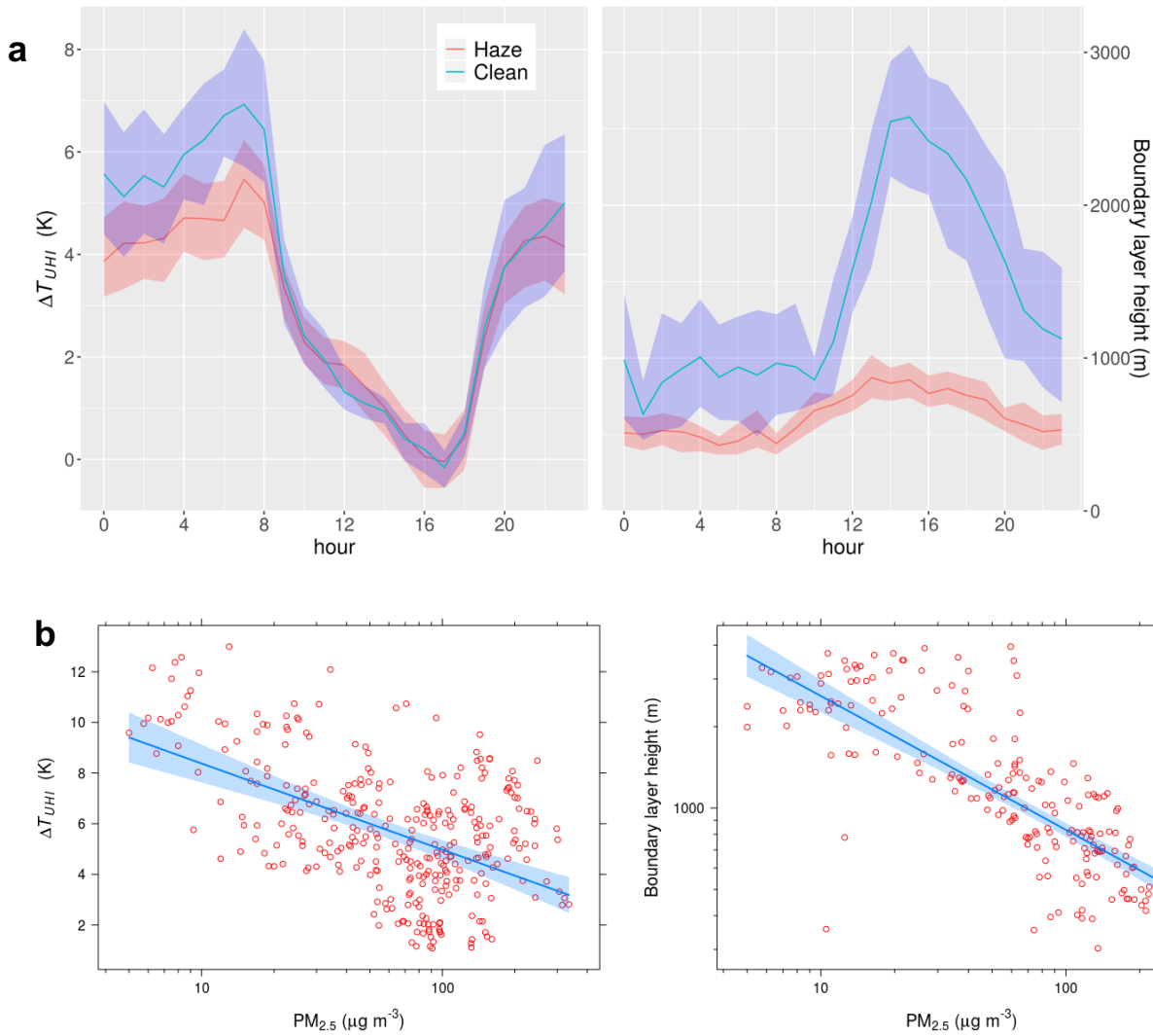
400 Figure 3: (a) Mean diurnal cycle of the magnitude of urban heat island ( \Delta T_{UHI} ) and boundary layer (BL) height during haze (30 days) and clean conditions (24 days) between 6 February 2018 and 31 March 2018. The shaded areas are the 95% confidence intervals of the fitted curve. \Delta T_{UHI} is calculated as a difference of air temperature between the Beijing University of Chemical Technology (BUCT) and rural station at south-east of Beijing (Daxing, 39.654 °N, 116.695 °E, see Ma, et al., 2018). (b) Scatter plots of boundary layer height versus PM_{2.5} concentration for daytime (hours 14–18) (right panel) and urban heat island magnitude ( \Delta T_{UHI} ) versus PM_{2.5} concentration for nighttime (hours 0–8) (left panel). The values where \Delta T_{UHI} is under 4 K with low PM_{2.5} concentrations (<40) has been filtered out since those low values of \Delta T_{UHI} are presumably caused by other phenomena than haze (e.g. cloudiness). The shaded areas indicate 95% confidence intervals.
