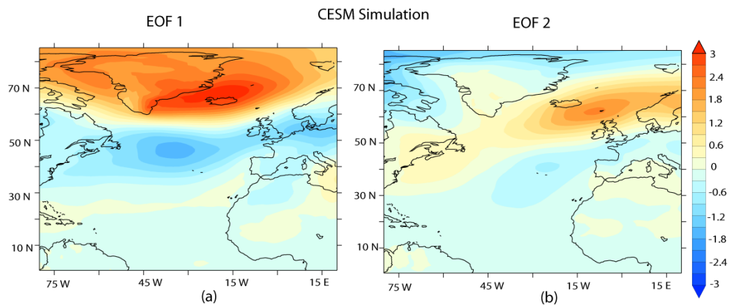
Fig. S2 EOFs of summer sea level pressure constructed using CESM Ctrl simulation for model years 0006-0015. EOF1 shows the summer NAO pattern and EOF2 shows SEA pattern.
