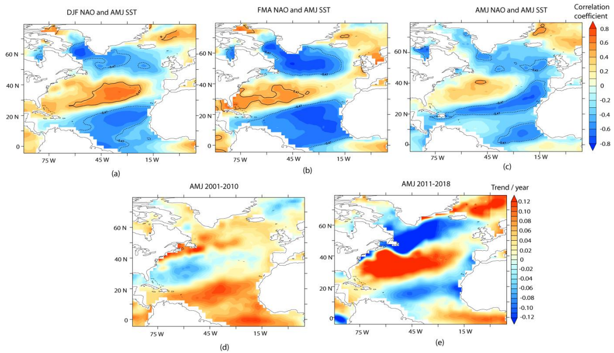
Fig. S1 Correlation between April-June North Atlantic SST and NAO index for (a) December-February, (b) February-April and (c) April-June for 2001-2018. Continuous (dashed) contours enclose the regions which have positive (negative) correlation coefficients significant at 95% confidence level. (d) and (e) Trends in April-June SST over the North Atlantic for 2001-2010 and 2011-2018.
