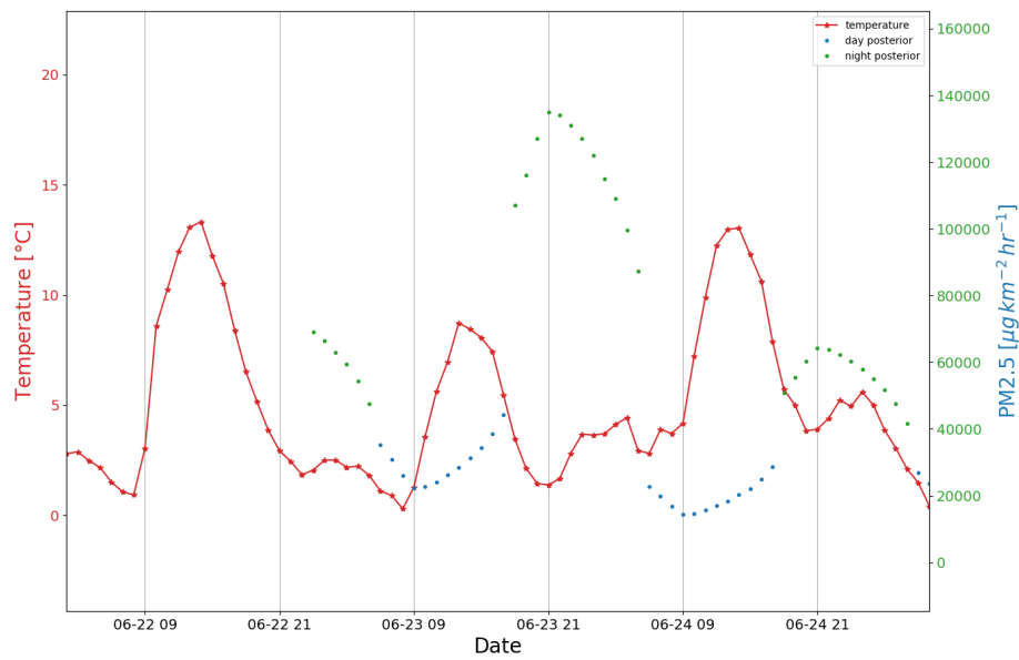
Figure 7. Hourly mean temperature as obtained from the AWS located at Kyle Street, together with the sum of the inferred PM_{2.5} emissions for day-time (blue) and night-time (green).
