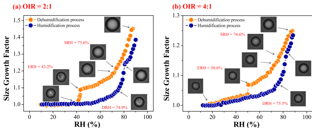
465 Figure 6: Hygroscopic cycles of mixed 1, 2, 6-hexanetriol/AS particles with OIR = 2:1 (a) and 4:1 (b). The panels show the optical images corresponding to the GFs at the certain RH. The SRH, ERH and DRH values are given in red.
