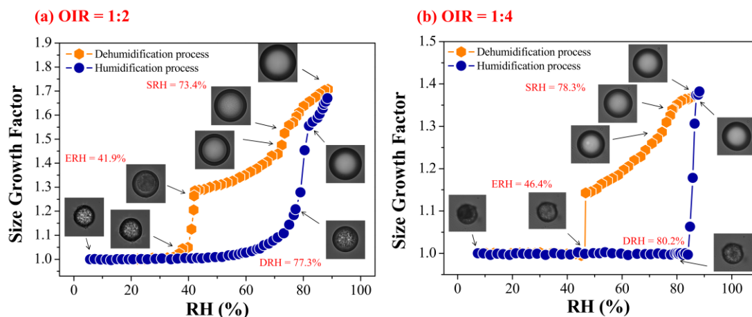
Figure 4: Hygroscopic cycles of mixed 1, 2, 6-hexanetriol/AS particles with OIR = 1:2 (a) and 1:4 (b). The panels show the optical images corresponding to the GFs at the certain RH. The SRH, ERH and DRH values are given in red.
