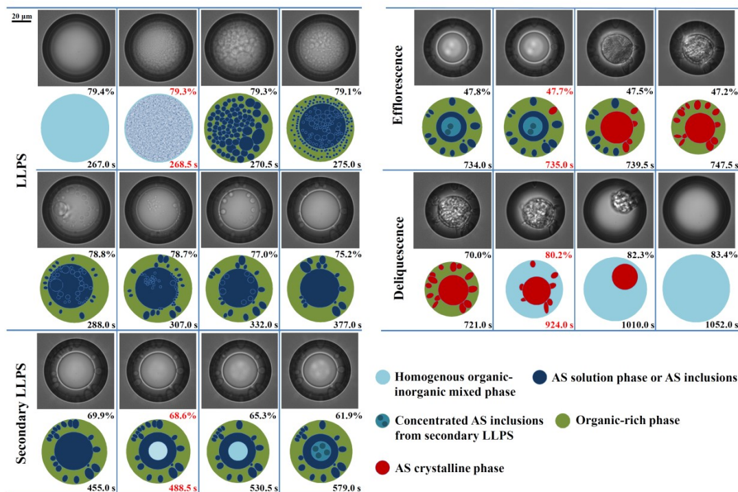
Figure 2: Optical images and corresponding illustrations of mixed 1, 2, 6-hexanetriol/AS particle with OIR = 1:1 during LLPS, secondary LLPS, efflorescence and deliquescence. Below the optical images are the illustrations. The corresponding RH and time are given in each frame. The RH and time in red indicate the occurrence of phase transitions.
