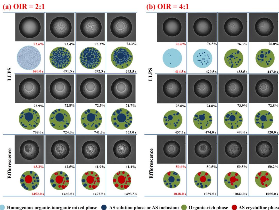
Figure 7: Optical images and corresponding illustrations of mixed 1, 2, 6-hexanetriol/AS particles with OIR = 2:1 (a) and 4:1 (b) during LLPS and efflorescence. Below the optical images are the illustrations. The corresponding RH and time are given in each frame. The RH and time in red indicate the occurrence of phase transitions.
