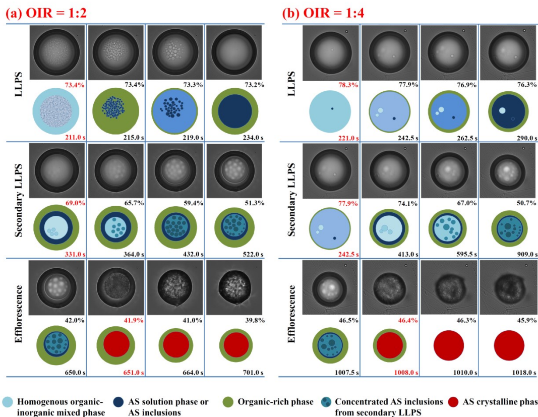
460 Figure 5: Optical images and corresponding illustrations of mixed 1, 2, 6-hexanetriol/AS particles with OIR = 1:2 (a) and 1:4 (b) during LLPS, secondary LLPS and efflorescence. Below the optical images are the illustrations. The corresponding RH and time are given in each frame. The RH and time in red indicate the occurrence of phase transitions.
